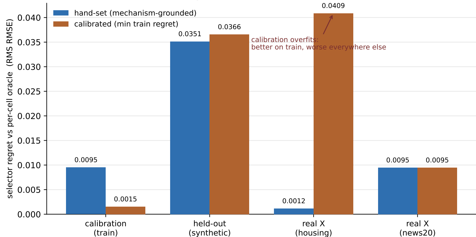
Mechanism-grounded thresholds generalise; tuned ones overfit multi-selector regret, thresholds calibrated on train vs hand-set
