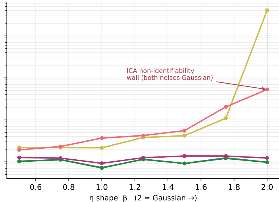
Gaussian \varepsilon ( \beta=2 )
