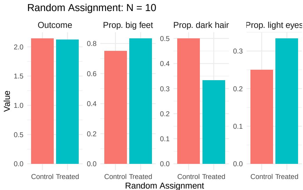
Figure 2.5: Random assignment with N=10. Some imbalance remains due to small sample size.
