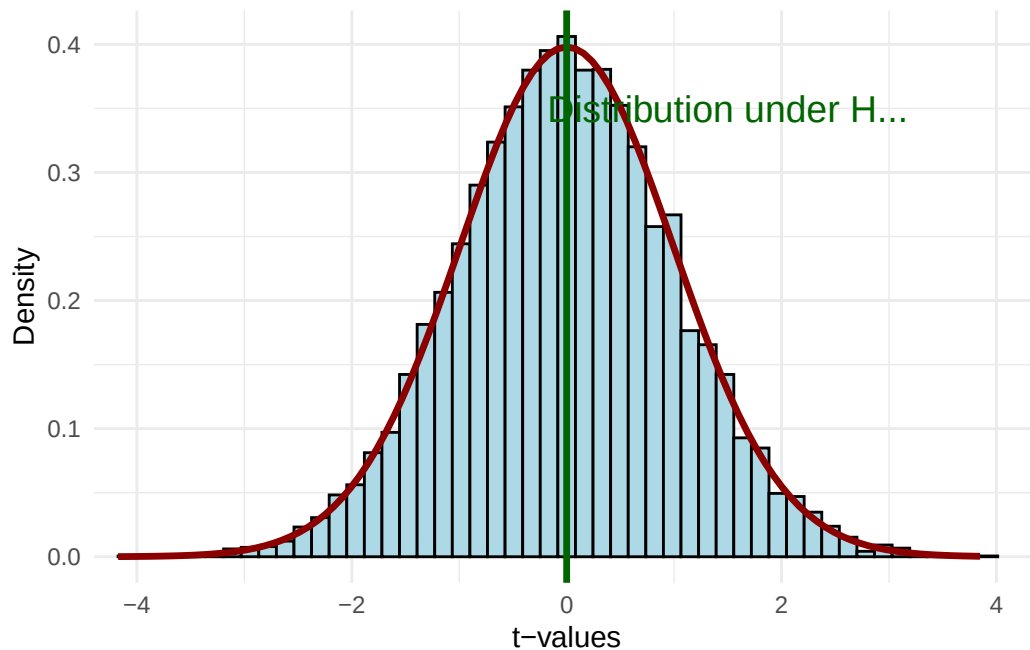
Figure 5.6: The t-distribution under the null hypothesis H_0: \mu = 0 . Most estimates will fall near zero.
