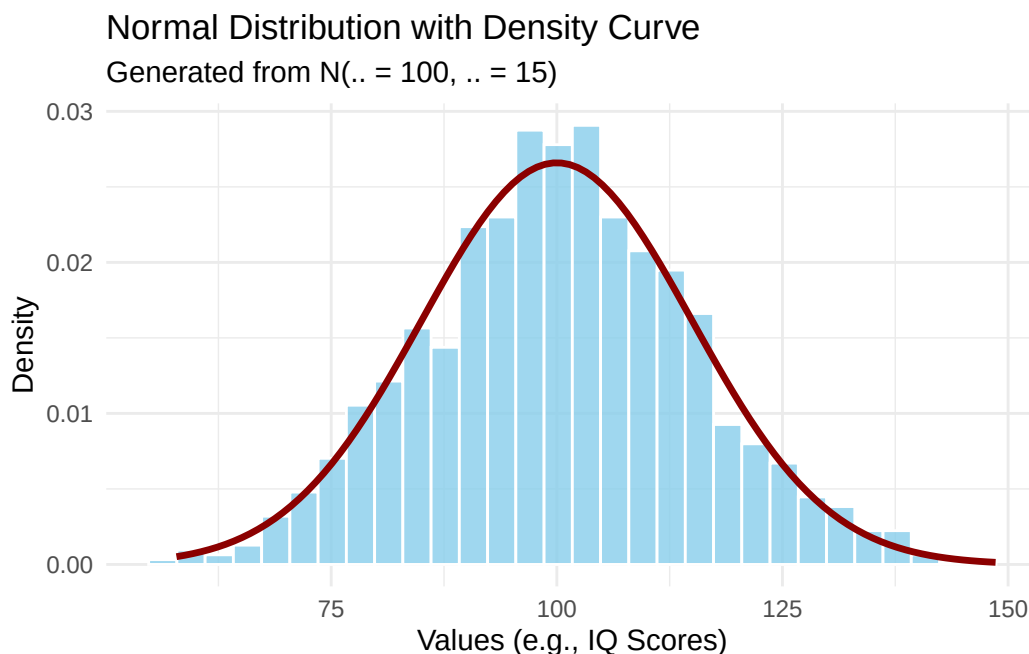
Figure 5.4: The normal (Gaussian) distribution—the classic ‘bell curve.’ The example shows IQ scores, which are designed to follow N(100, 15) .
