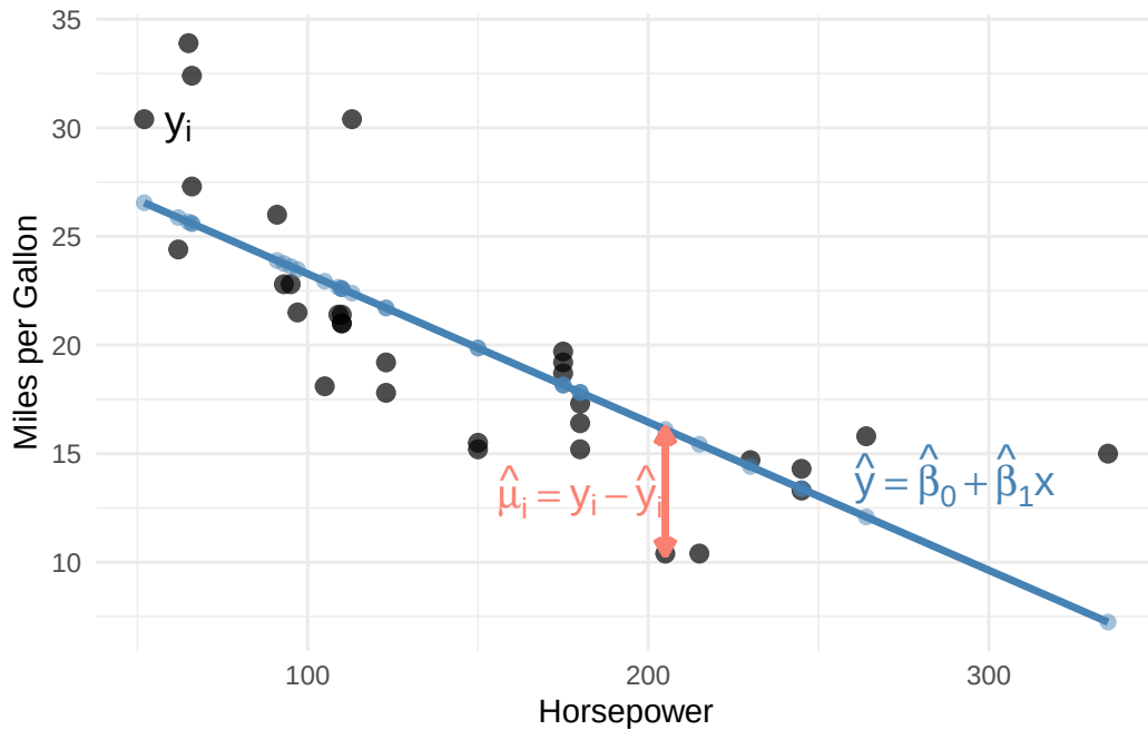
Figure 3.2: Components of the regression line. Black points show actual values, the blue line shows predicted values, and the salmon segment illustrates a residual.
