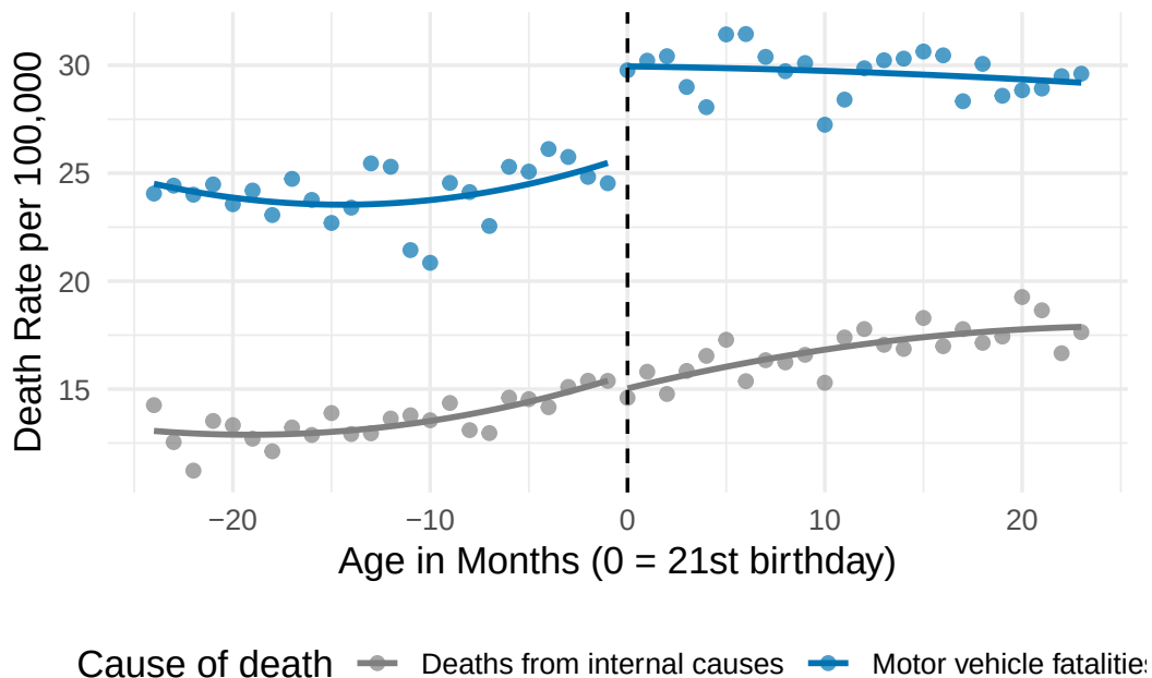
Figure 15.6: A visual falsification test: motor vehicle fatalities (blue) jump sharply at the MLDA cutoff, while deaths from internal causes (gray) show essentially no jump. This pattern supports a causal interpretation of the MLDA effect.
