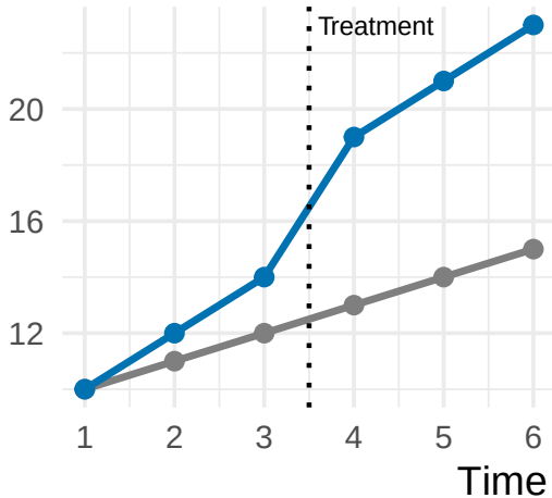
Diverging Pre-Trends (Bad)
