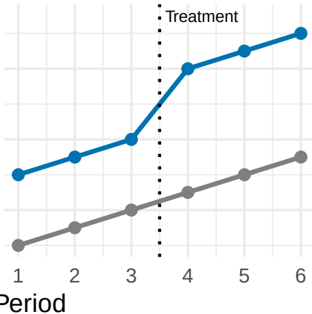
Parallel Pre-Trends (Good)
