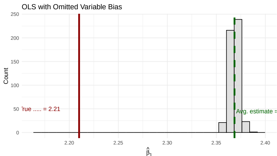
Figure 3.5: With omitted variable bias, the average of OLS estimates (green) systematically differs from the true value (red). The bias persists even with many samples.
