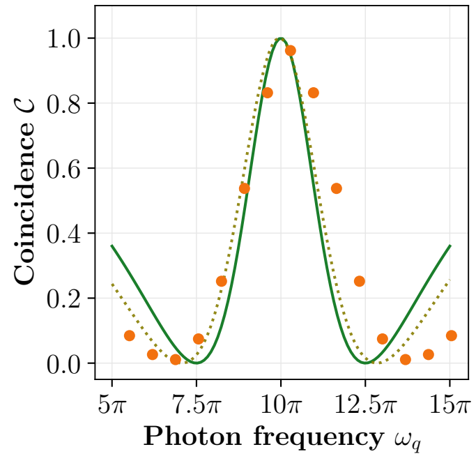
(a) \omega_{\text{ref}} = 10\pi , \Lambda = 10\pi
