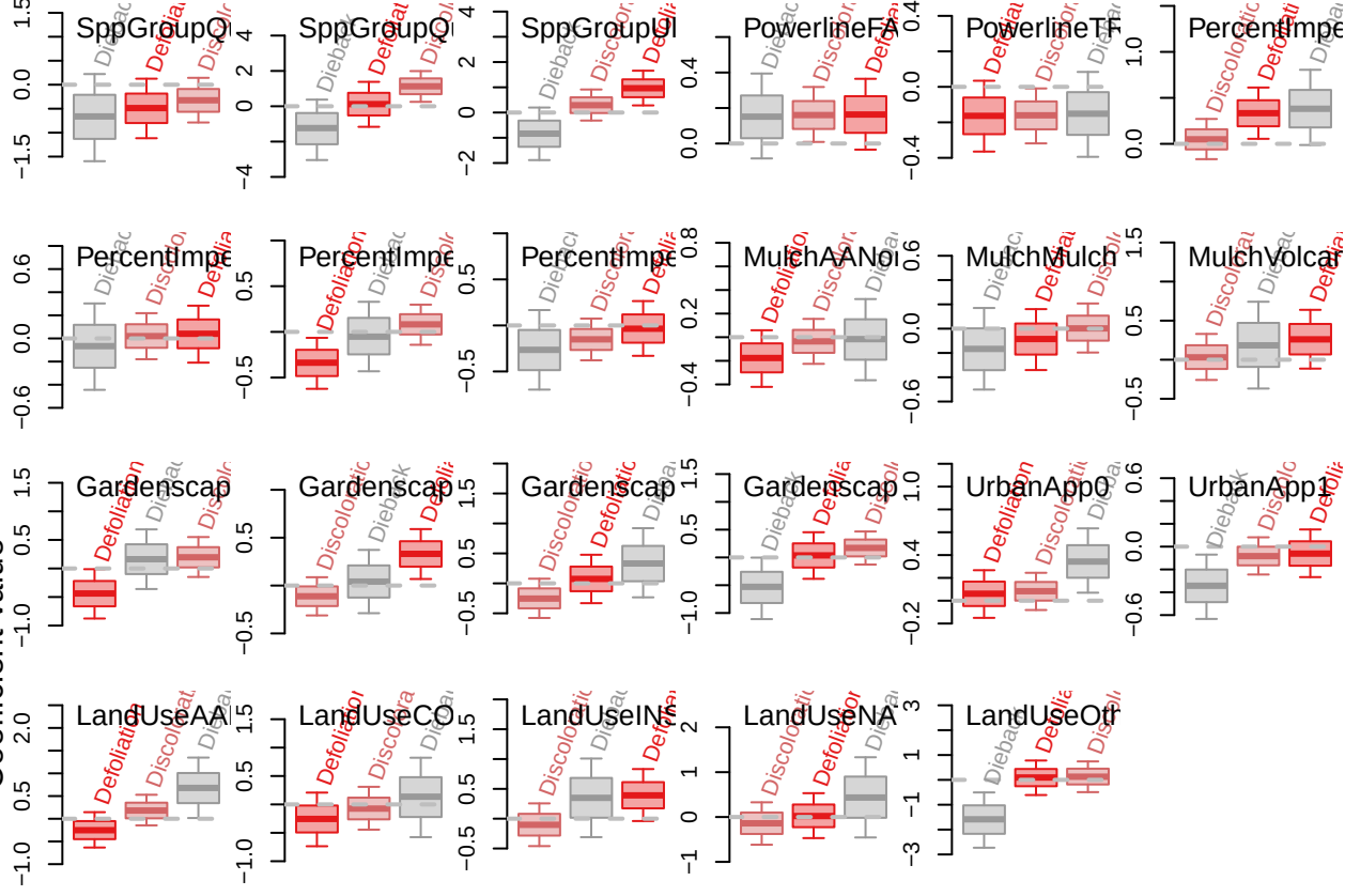
Coefficient value
