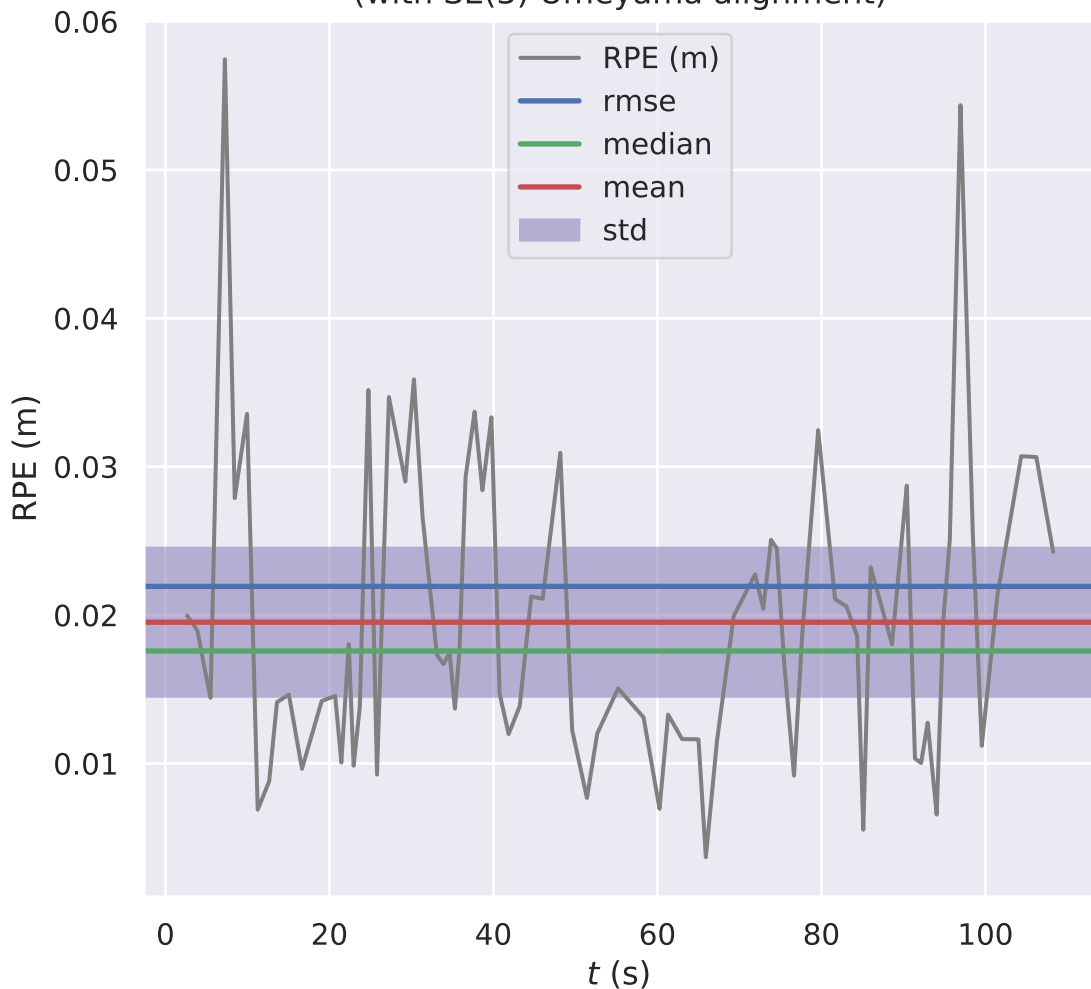
RPE w.r.t. translation part (m) for \delta = 1.0 (m) using consecutive pairs (with SE(3) Umeyama alignment)
