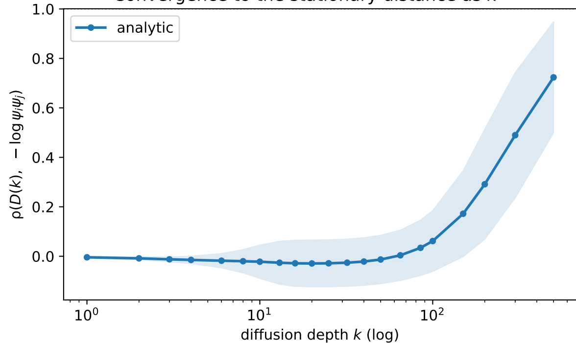
Convergence to the stationary distance as k \rightarrow \infty
