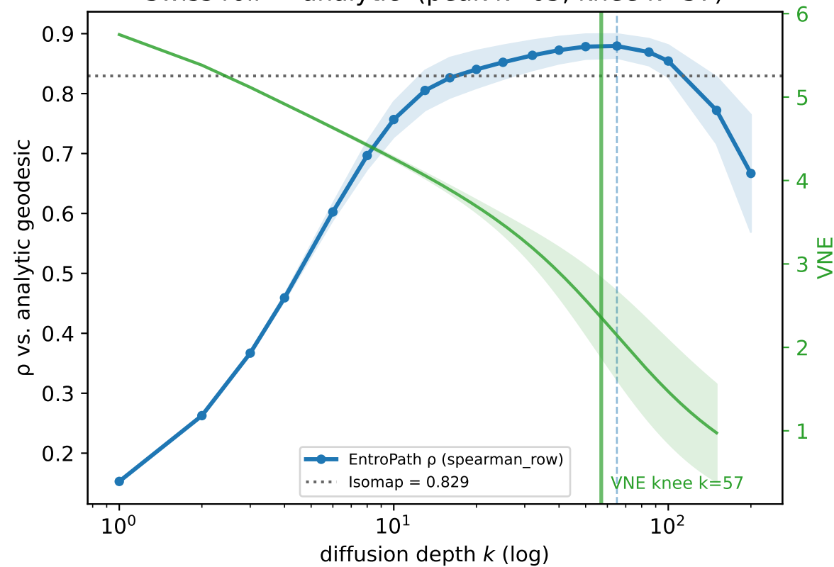
Swiss roll — analytic (peak k=65 , knee k=57 )
