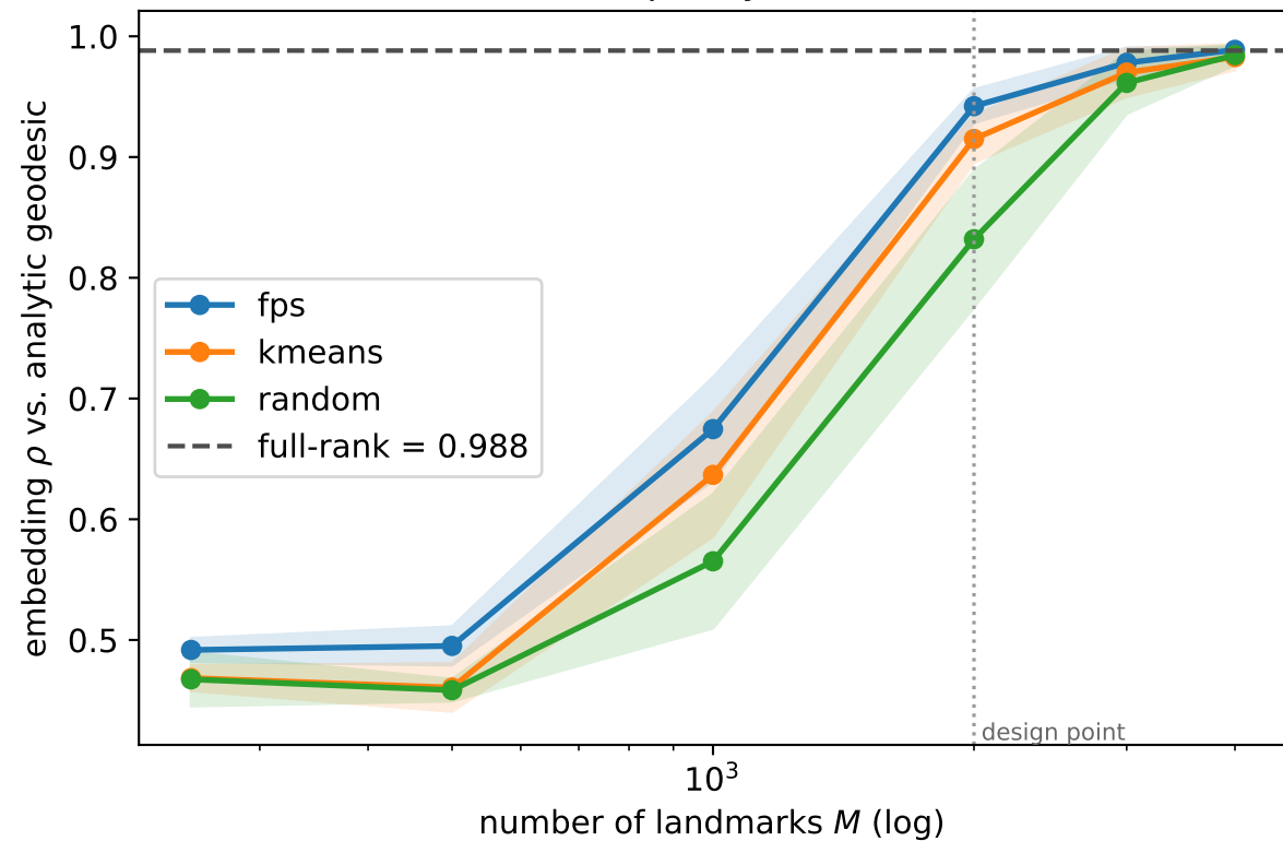
Landmark count vs. quality (Swiss roll, N = 5000 )
