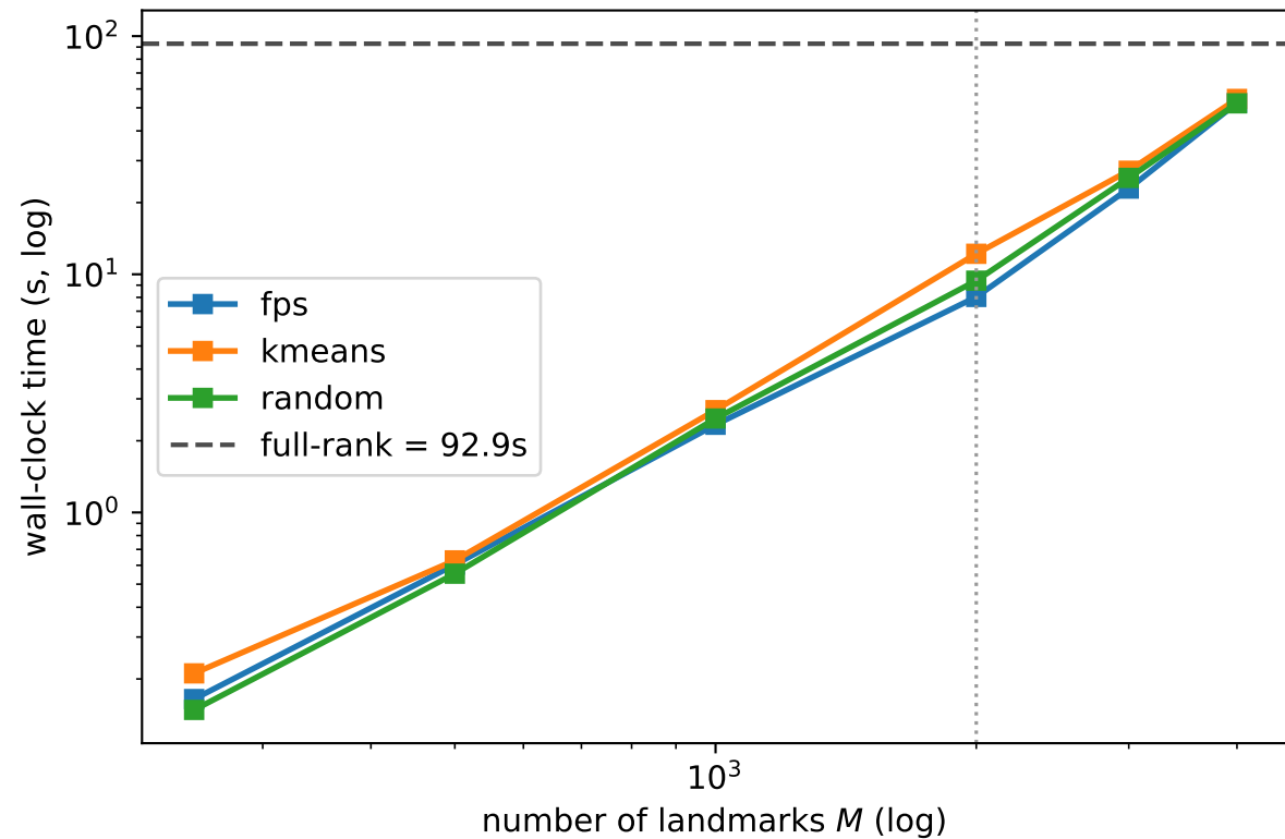
Landmark count vs. runtime (Swiss roll, N = 5000 )
