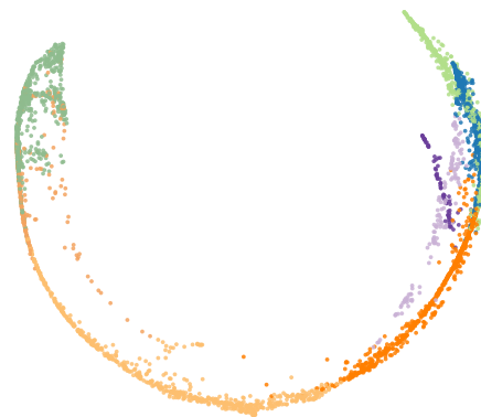
PHATE
