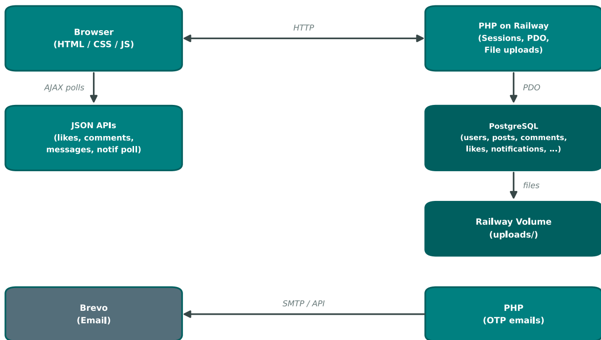
Figure 1. Runtime architecture of BondNest showing browser, PHP server, PostgreSQL, uploads, and Brevo email service.
