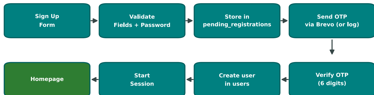
Figure 2. Registration and email OTP verification workflow.
