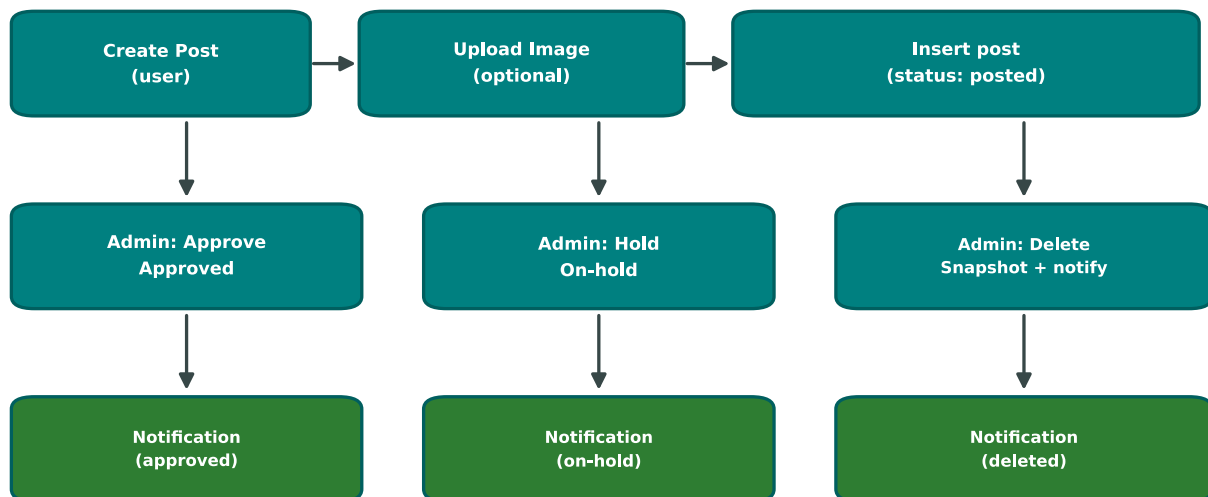
Figure 4. Posting and moderation workflow.
