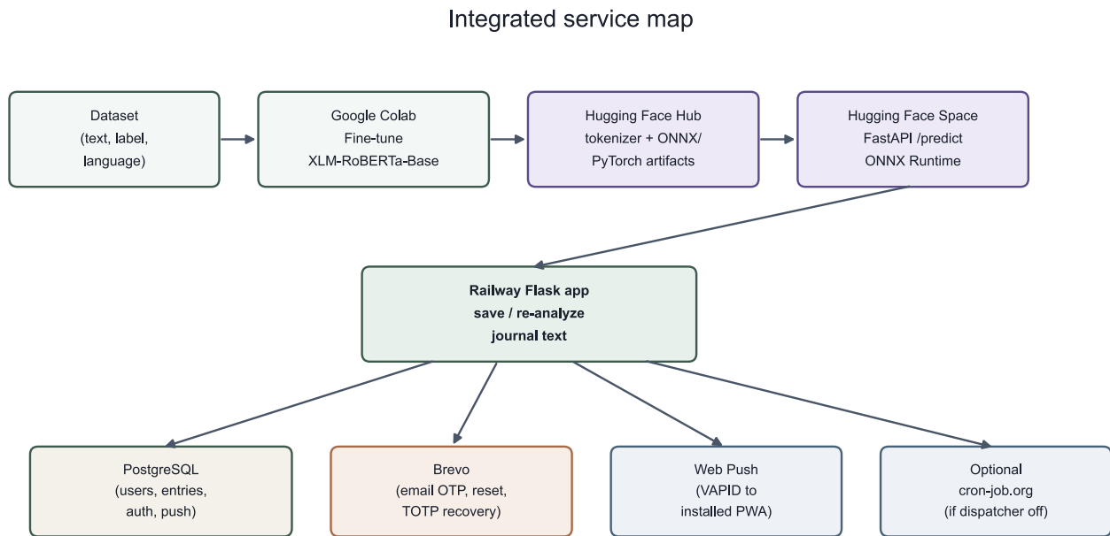
Figure 3. Integrated service map showing the training-to-inference pipeline and supporting services.
