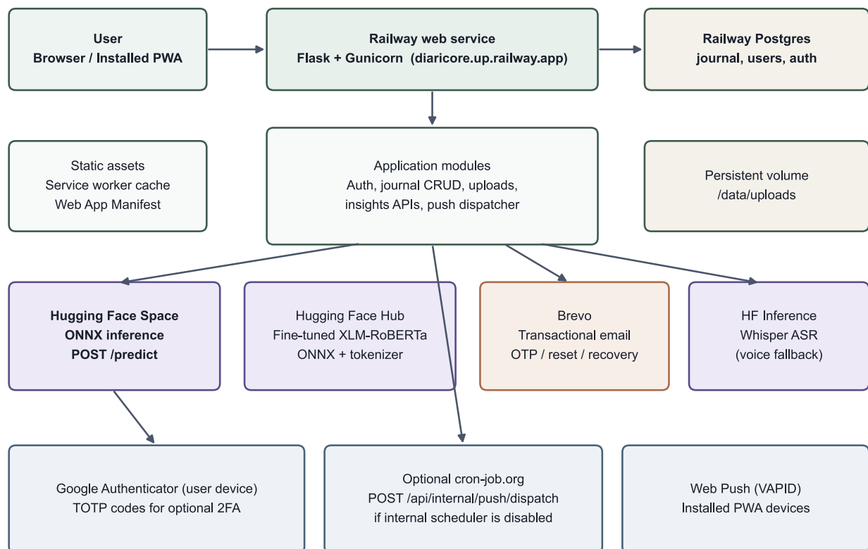
DiariCore — current runtime architecture
