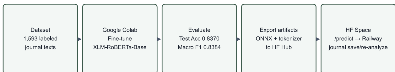
Figure 11. Training-to-inference workflow used by the current system.
