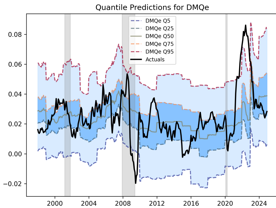
Figure 1: Forecasts for Infl_yoy using DMQe
