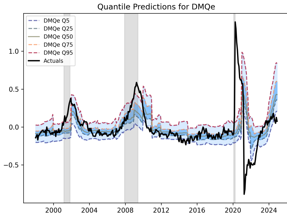
Figure 3: Forecasts for Unrate_yoy using DMQe
