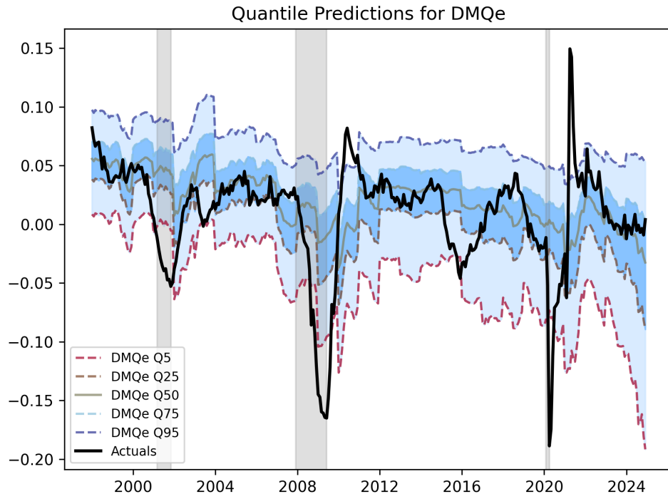
Figure 2: Forecasts for IP_yoy using DMQe
