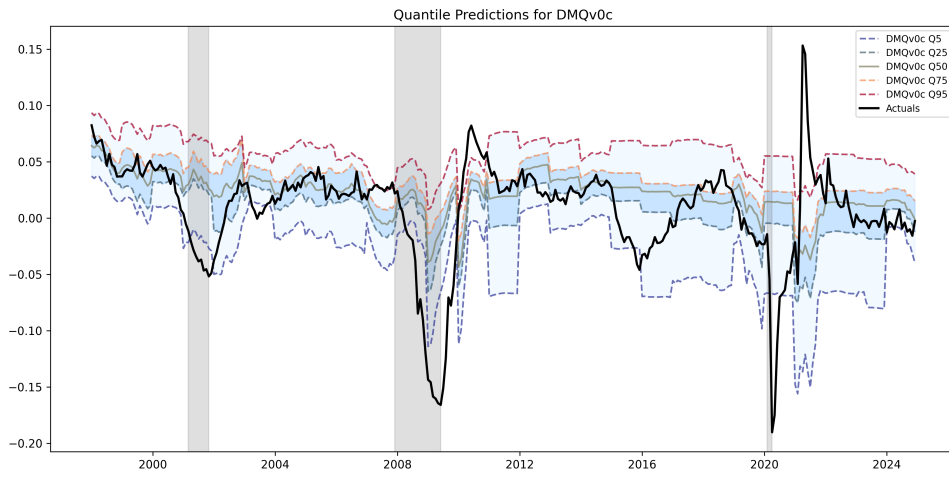
Figure 2: Forecasts for IP_yoy using DMQv0c
