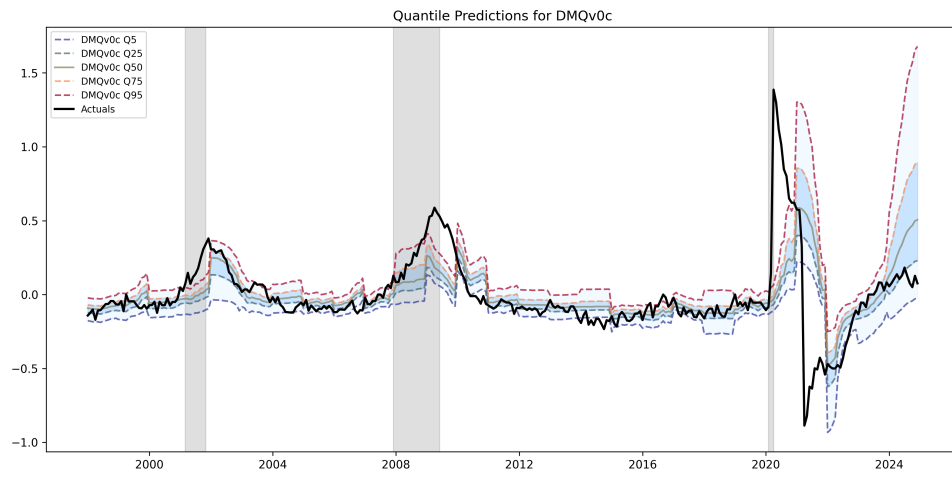
Figure 3: Forecasts for Unrate_yoy using DMQv0c
