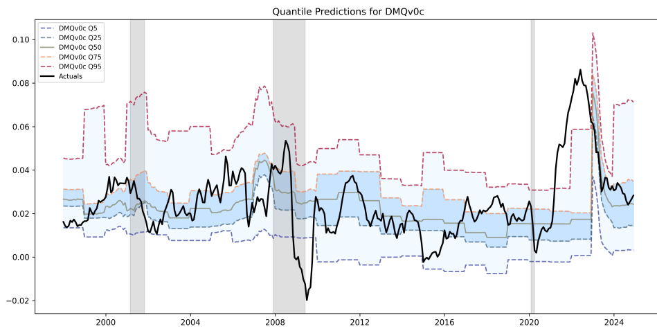
Figure 1: Forecasts for Infl_yoy using DMQv0c
