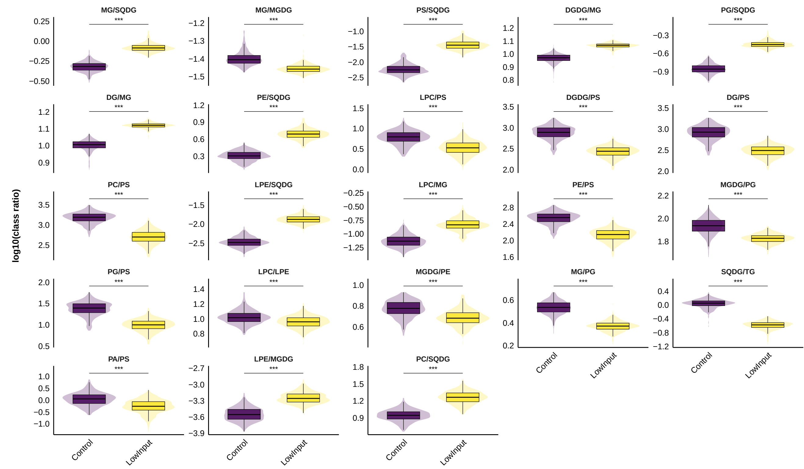
A) OPLS-DA Discriminatory Ratios (log10 scale)
