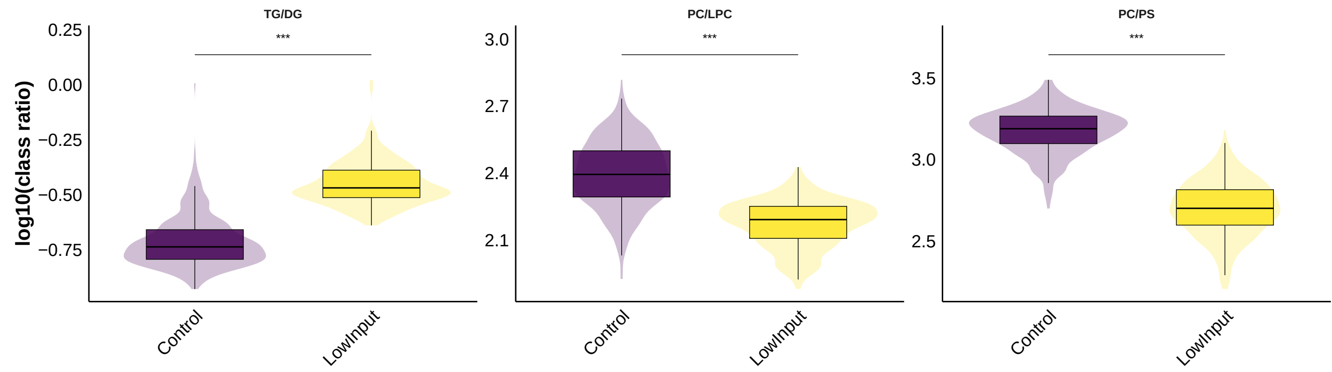
B) Correlation-Derived Ratios (log10 scale)
