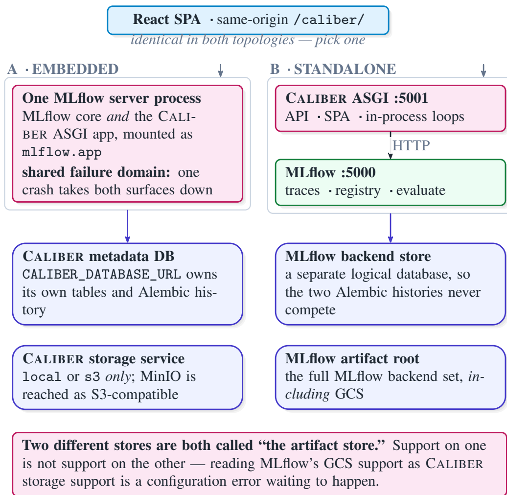
Figure 9: The two deployment topologies. One ASGI application, two ways to run it; the API and the SPA are identical, so the choice is a failure-domain and operations decision rather than a feature one. Topology A mounts CALIBER inside the MLflow server process as an mlflow.app , which is convenient for development and couples the two failure domains. Topology B runs CALIBER as its own service reaching a vanilla MLflow over HTTP. In neither mode is CALIBER a transparent gateway in front of MLflow: it is a sibling surface, not a proxy. Two configuration facts are called out because both are load-bearing and both are easy to get wrong. CALIBER_DATABASE_URL independently owns CALIBER’s tables and is not required to equal MLflow’s backend store — the bundled stack uses separate logical databases precisely so the two Alembic histories never compete for one version table. And “artifact store” names two different things: MLflow’s artifact root supports its full backend set including GCS, while CALIBER’s own storage service accepts local and s3 only.
