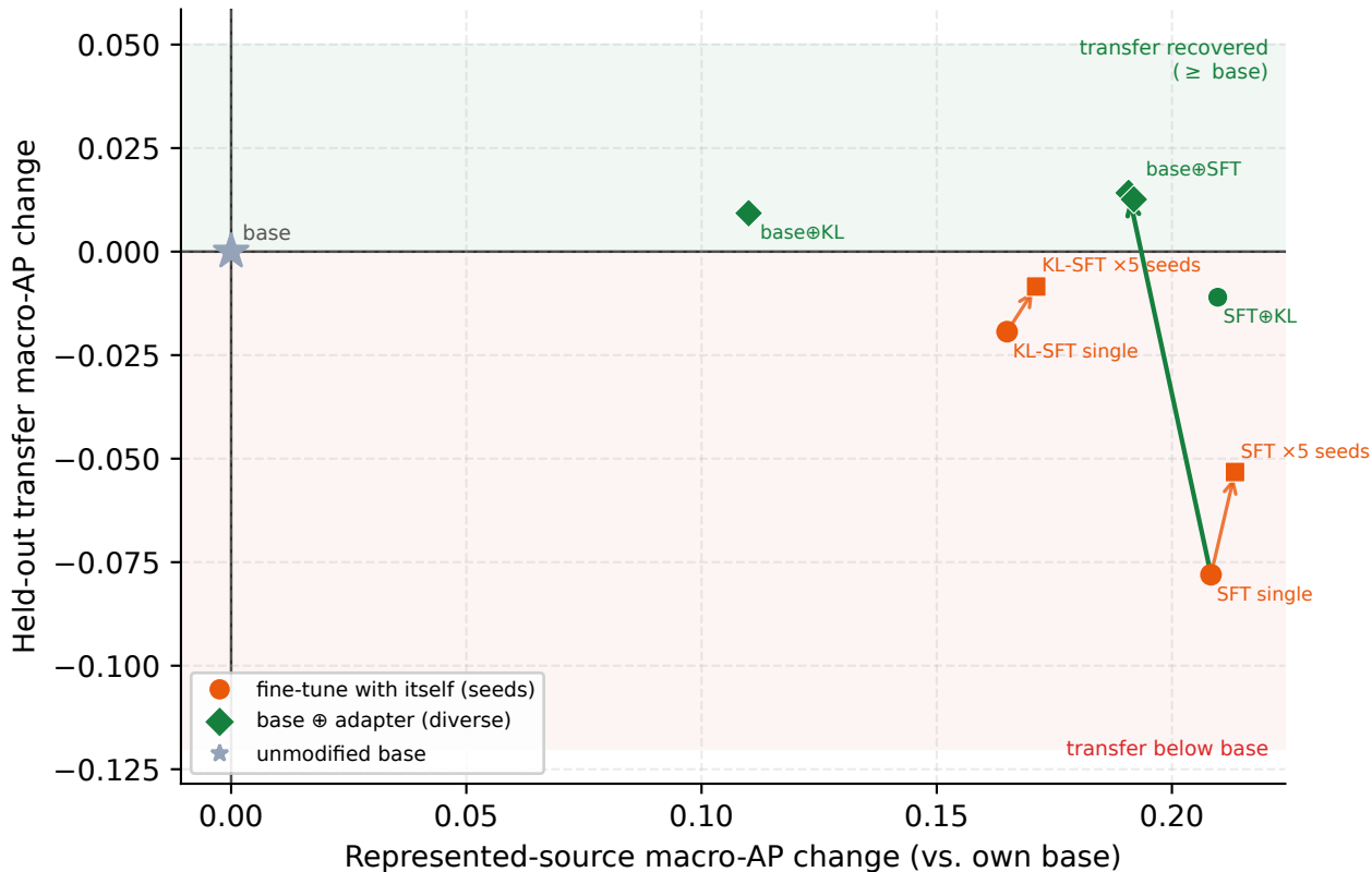
Ensembling plane: only crossing the specialization axis recovers transfer
