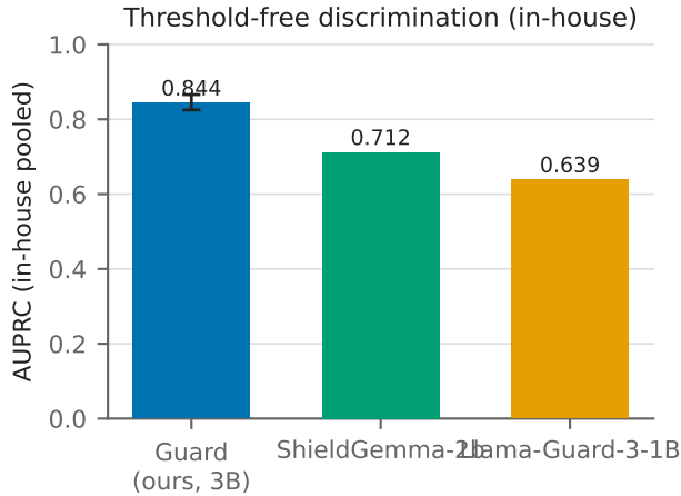
Figure 3: Pooled in-house AUPRC (2,018 test rows): the guard (0.844) leads ShieldGemma-2b (0.712) and Llama-Guard-3-1B (0.639) on point estimates.
