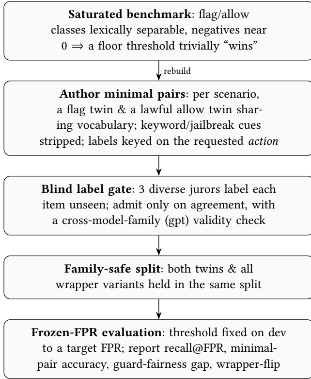
Figure 7: Turning a saturated benchmark into a hardened, minimal-pair rebuild and scoring it (§6.2). Technique only; result magnitudes are in Table 11.
