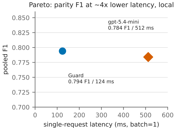
Figure 5: F1 versus single-request (batch=1) latency: the guard sits at parity with gpt-5.4-mini on F1 at roughly 4x lower latency (124 ms vs ~512 ms per request).
