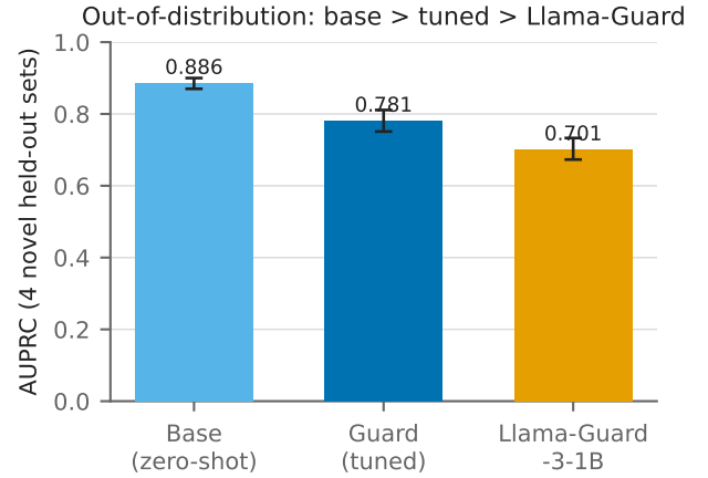
Figure 4: Aggregate AUPRC on the novel held-out benchmarks (2,020 balanced rows): the zero-shot base (0.886) out-ranks the tuned guard (0.781), which in turn beats Llama-Guard-3-1B (0.701), with non-overlapping 95% CIs.
