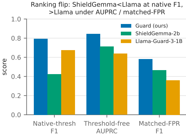
Figure 8: ShieldGemma-2b vs Llama-Guard-3-1B under native-threshold F1, threshold-free AUPRC, and matched-FPR@0.10: the native-F1 ranking inverts under both operating-point-fair metrics.
