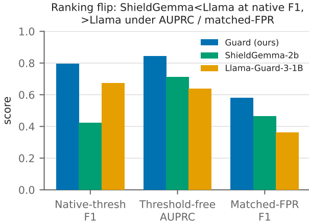
Figure 9: ShieldGemma-2b vs Llama-Guard-3-1B under native-threshold F1, threshold-free AUPRC, and matched-FPR@0.10: the native-F1 ranking inverts under both operating-point-fair metrics.
