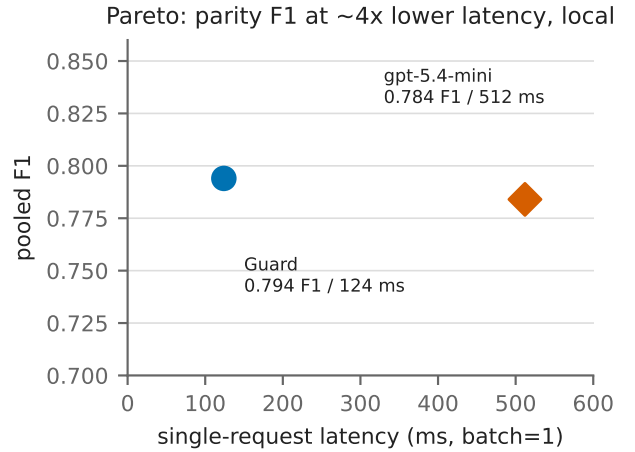
Figure 6: F1 versus single-request (batch=1) latency: the guard sits at parity with gpt-5.4-mini on F1 at roughly 4x lower latency (124 ms vs ~512 ms per request).
