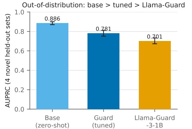
Figure 5: Aggregate AUPRC on the novel held-out benchmarks (2,020 balanced rows): the zero-shot base (0.886) out-ranks the tuned guard (0.781), which in turn beats Llama-Guard-3-1B (0.701), with non-overlapping 95% CIs.
