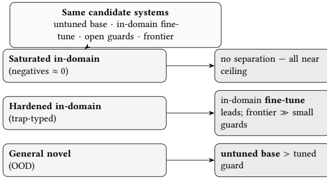
Figure 7: The benchmark chooses the winner. The identical systems yield a different verdict per regime: a saturated benchmark separates nobody; a hardened in-domain rebuild is led by the in-domain fine-tune, with a frontier model far ahead of every small guard; and on general out-of-distribution benchmarks the untuned base outranks the tuned guard (§6.1, §6.2).
