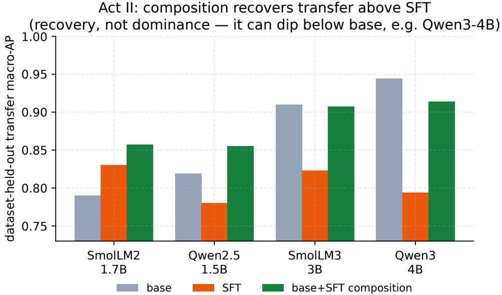
Figure 6: Per-checkpoint transfer macro-AP for base, SFT, and the base+SFT composition. Composition (green) exceeds SFT (orange) for every checkpoint; relative to the base it lands above for the two weaker bases, approximately at base for SmolLM3-3B (0.907 vs. 0.910), and below base for the strongest base (Qwen3-4B) — transfer recovery , not Pareto dominance.
