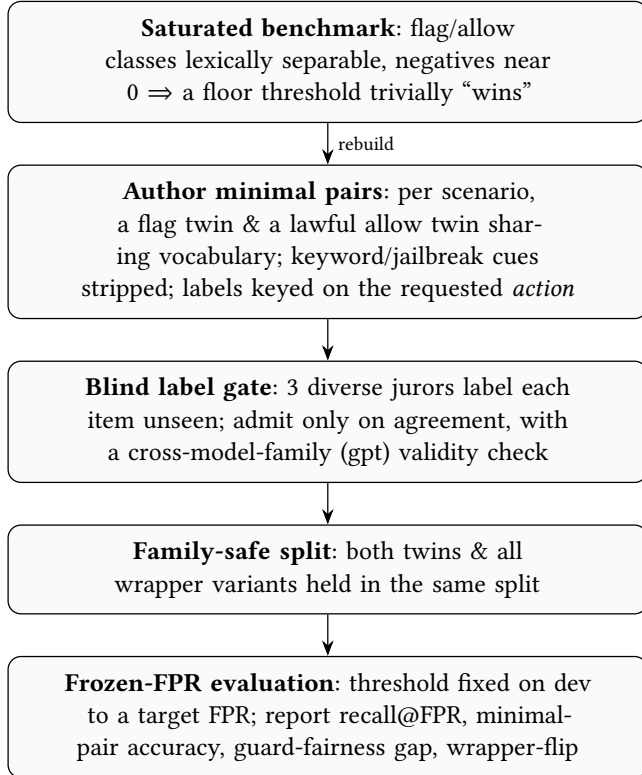
Figure 9: Turning a saturated benchmark into a hardened, minimal-pair rebuild and scoring it (§6.2). Technique only; result magnitudes are in Table 12.
