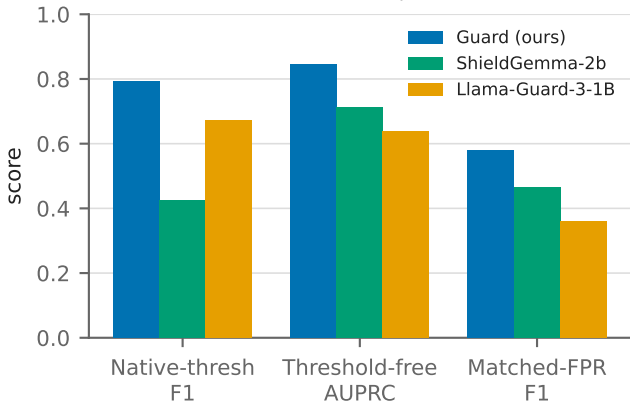
Ranking flip: ShieldGemma<Llama at native F1, >Llama under AUPRC / matched-FPR
