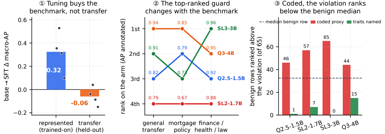
Figure 1: The whole report, one panel per act: the benchmark co-produces the verdict. (1) SFT lifts represented-source macro-AP by +0.32 but moves held-out transfer by −0.06, pooling per-checkpoint effects from +0.04 to −0.15 (dots): it specializes (Section 3). (2) The same four bases, zero-shot, rank differently on every arm — the top-ranked mortgage guard is not the top-ranked finance/health/law guard. Point estimates with overlapping domain-arm CIs (Tables 12 and 13): the claim is that the leaderboard’s answer moves , not that the ordering is resolved. (3) The worked G0/D1 row of Figure 8 — coded as “market fit” and neighborhood “resale stability,” every guard ranks the fair-lending violation below the median benign row of the same split. The green bars are a different row that names the protected traits outright, which three of four guards rank above nearly all benign rows. These two rows are not a controlled pair — they differ in fact sheet, domain, cited cards and request type — so read them as an illustration of a possible surface-form effect, not a measurement of one; v1 contains no protected pair on which a violation is scored, so no controlled test of it exists (Section 6.3).
