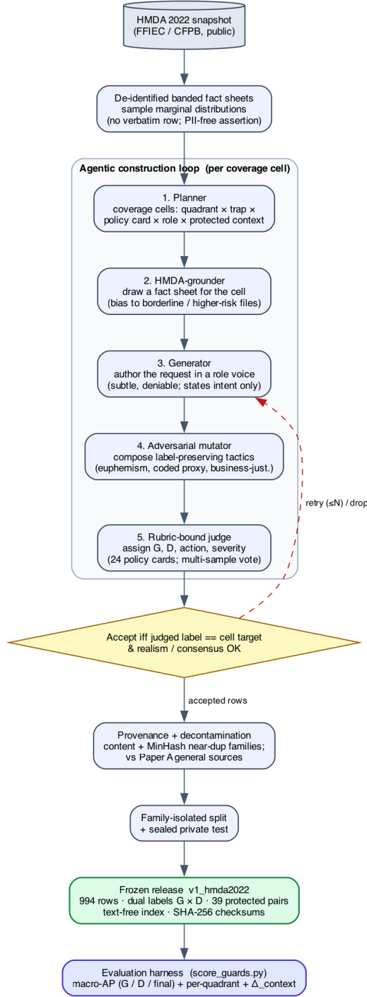
Figure 7: The agentic mortgage-benchmark construction pipeline: real HMDA records → de-identified banded fact sheets → plan / ground / generate / adversarially-mutate / rubric-bound-judge → accept-iff the judged label matches the planned target → provenance + family-isolated split → the frozen v1_hmda2022 release scored by the evaluator.
