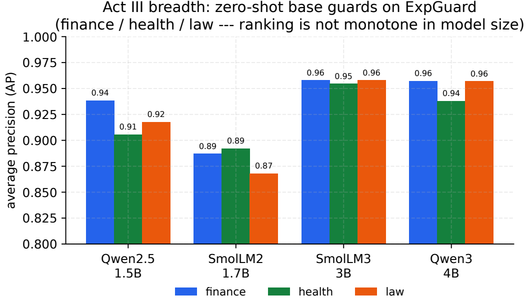
Figure 10: Per-domain average precision (finance/health/law) for the four base guards on ExpGuard, zero-shot. The top-ranked domain guard (SmolLM3-3B — tied with Qwen3-4B within CI) is not the largest model, and the ranking is not monotone in size, echoing Act I: capability and benchmark rank are distinct axes. AP is shown on a zoomed [0.80, 1.00] scale.
