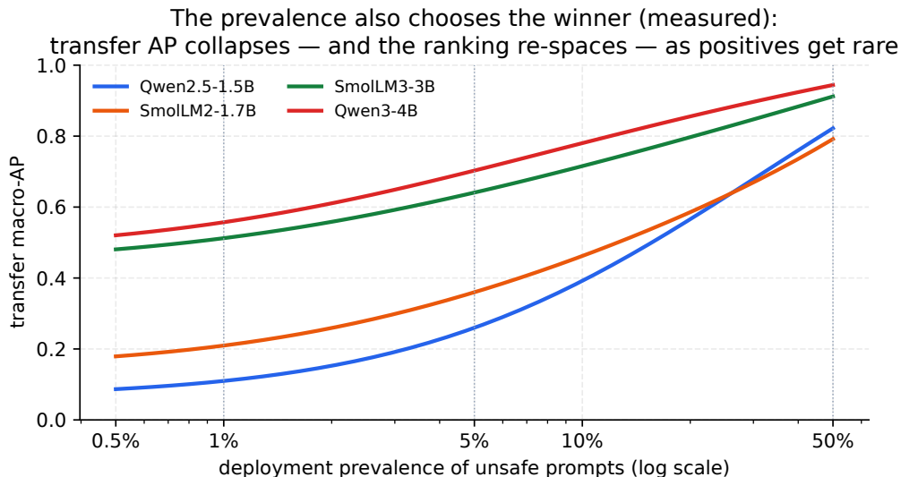
Figure 3: The prevalence also chooses the winner (measured: Equation (4) applied to the four base guards’ committed transfer ROC, macro-averaged over the transfer sources). As unsafe prompts get rarer, every guard’s AP falls — the strongest ranker (Qwen3-4B) drops from 0.94 at balance to \approx 0.56 at 1% prevalence, the weakest (Qwen2.5-1.5B) from 0.82 to 0.11 — and the lower half re-orders (see text).
