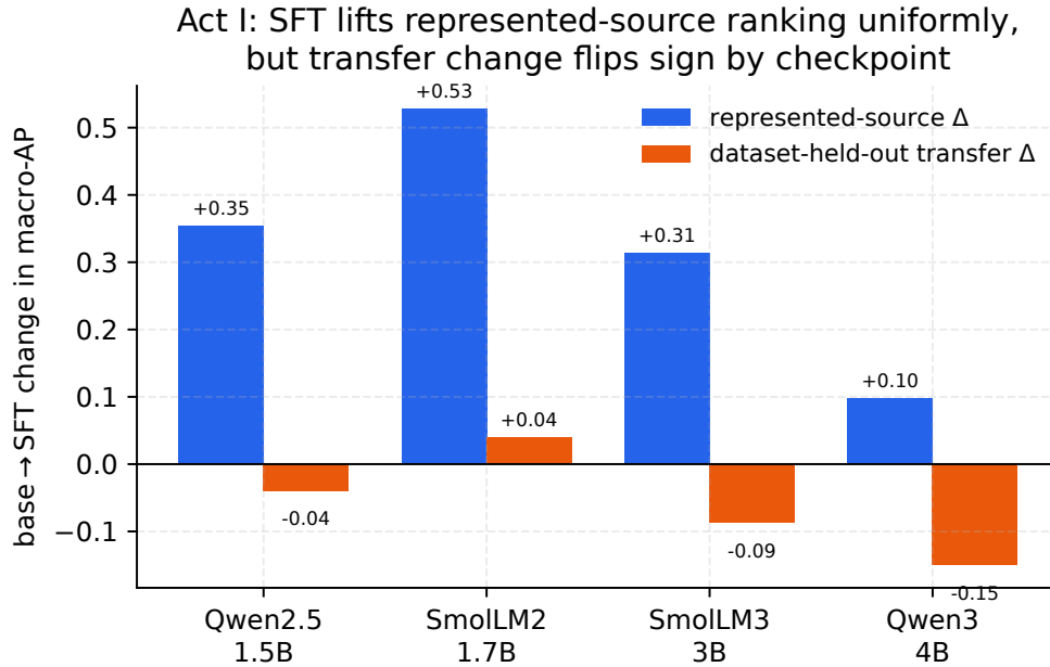
Figure 5: Per-checkpoint view of Act I: SFT lifts represented-source macro-AP for every checkpoint (blue), but the transfer change (orange) ranges from +0.04 (SmolLM2) to -0.15 (Qwen3-4B) — the fixed-panel average hides opposite signs.
