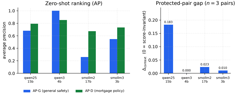
Figure 9: Zero-shot base guards on the mortgage benchmark: ranking (AP·G, AP·D; left) and the protected-pair fairness gap \Delta_{\text{context}} (right). AP·D is only moderate, and \Delta_{\text{context}} separates guards that AP alone rates similarly (Qwen2.5-1.5B’s 0.183 gap vs. Qwen3-4B’s 0).
