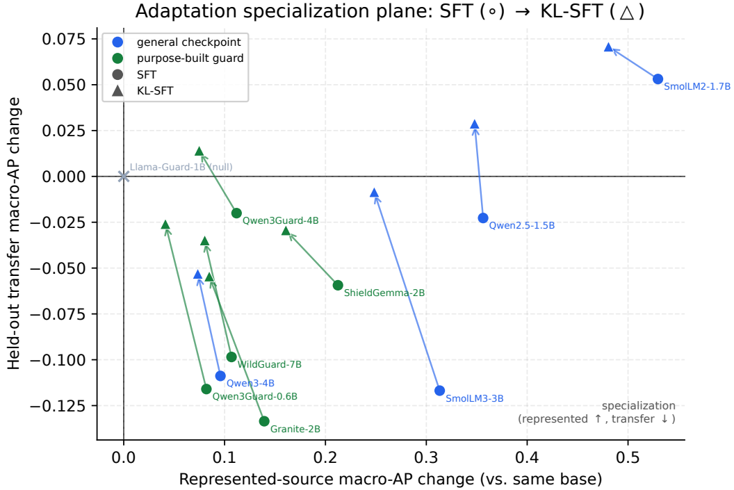
Figure 4: The adaptation specialization plane. Each checkpoint’s macro-AP change vs. its own unmodified base, on represented (x) and held-out transfer (y) sources, under SFT (◦) and KL-SFT (△); arrows run SFT → KL-SFT. Nearly all checkpoints — general (blue) and released purpose-built guards (green) alike — land in the specialization quadrant (represented up, transfer down: RQ1 ). The KL-SFT arrows point up-and-left: it recovers transfer at a represented-source cost ( RQ2 ). Llama-Guard-3-1B’s 20-token-pruned tied head is unmovable by LoRA (null cell at the origin).
