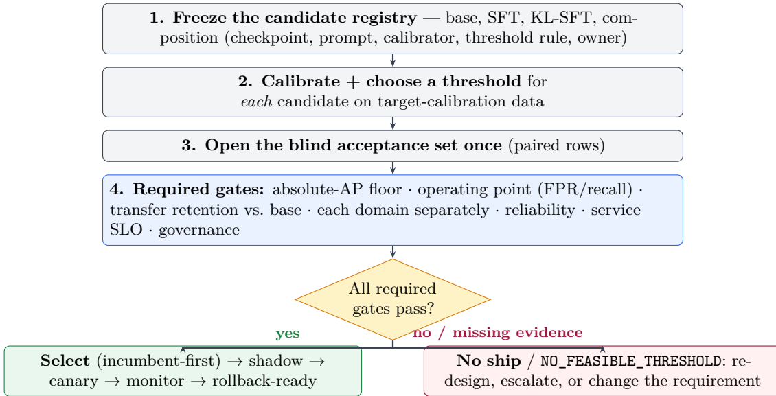
Figure 11: Gate candidates, not leaderboards (recommended workflow; not validated end to end by this study). Every candidate is calibrated and thresholded separately, evaluated once on a blind acceptance set, and must clear all required gates; a missing required gate is a failure, and an empty feasible set is a deliberate NO-SHIP, not a relaxed cutoff.
