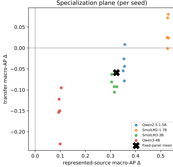
Figure 2: Each point is one (checkpoint, seed): horizontal axis is the represented-source macro-AP change, vertical axis the transfer change. 15/20 land in the lower-right specialization quadrant — the visual signature of Act I.
