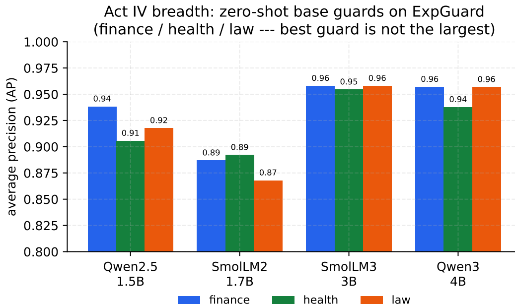
Figure 11: Per-domain average precision (finance/health/law) for the four base guards on ExpGuard, zero-shot. The best domain guard (SmolLM3-3B) is not the largest model, echoing Act I: capability and benchmark rank are distinct axes. AP is shown on a zoomed [0.80, 1.00] scale.
