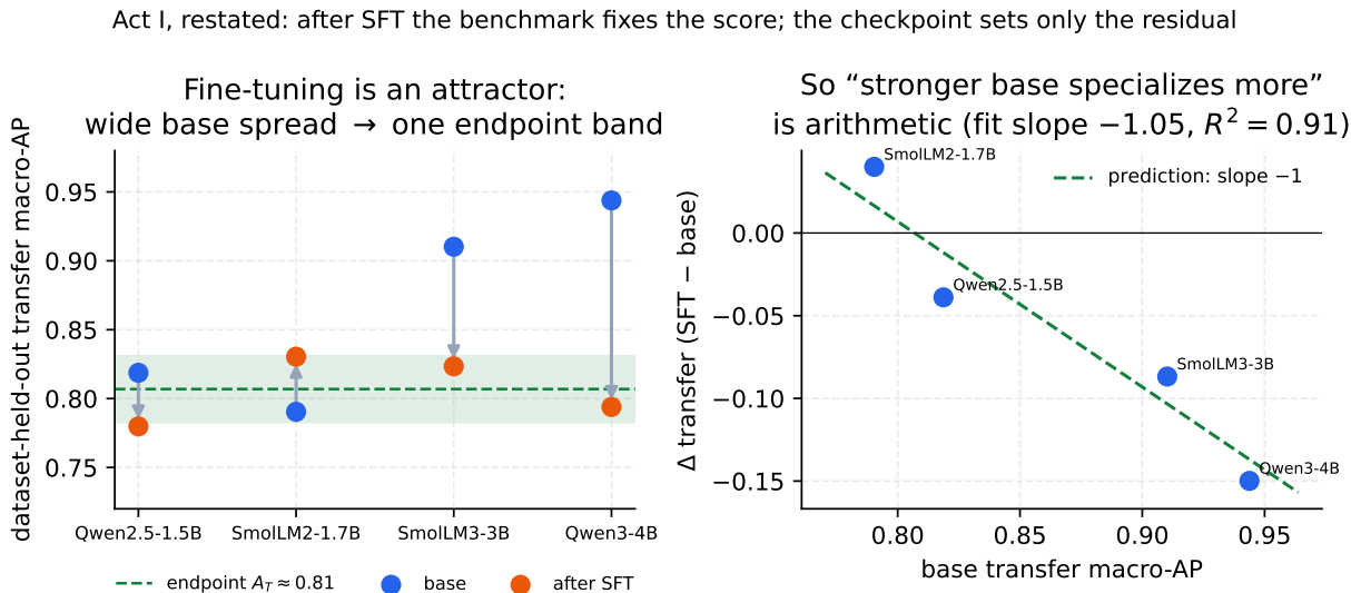
Figure 4: The fine-tuning attractor. Left: on the transfer benchmarks the four base checkpoints span 0.79–0.94 macro-AP, but after SFT they collapse into a narrow band around a benchmark-fixed endpoint A_T \approx 0.81 . Right: because every checkpoint lands near that same endpoint, the paired change \Delta = \text{SFT} - \text{base} is forced onto a line of slope -1 (green); the four points sit on it (fitted slope -1.05 , R^2 = 0.91 ). “Stronger bases specialize more” is therefore arithmetic, not a discovered behavioral law.
