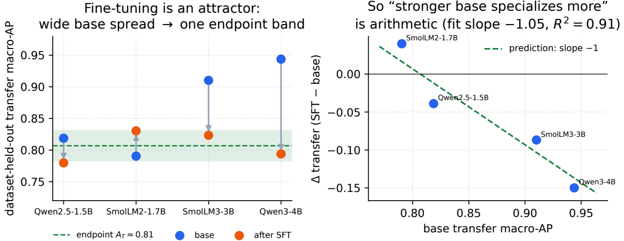
Figure 3: The fine-tuning attractor. Left: on the transfer benchmarks the four base checkpoints span 0.79–0.94 macro-AP, but after SFT they collapse into a narrow band around a benchmark-fixed endpoint A_T \approx 0.81 . Right: because every checkpoint lands near that same endpoint, the paired change \Delta = \text{SFT} - \text{base} is forced onto a line of slope -1 (green); the four points sit on it (fitted slope -1.05 , R^2 = 0.91 ). “Stronger bases specialize more” is therefore arithmetic, not a discovered behavioral law.
