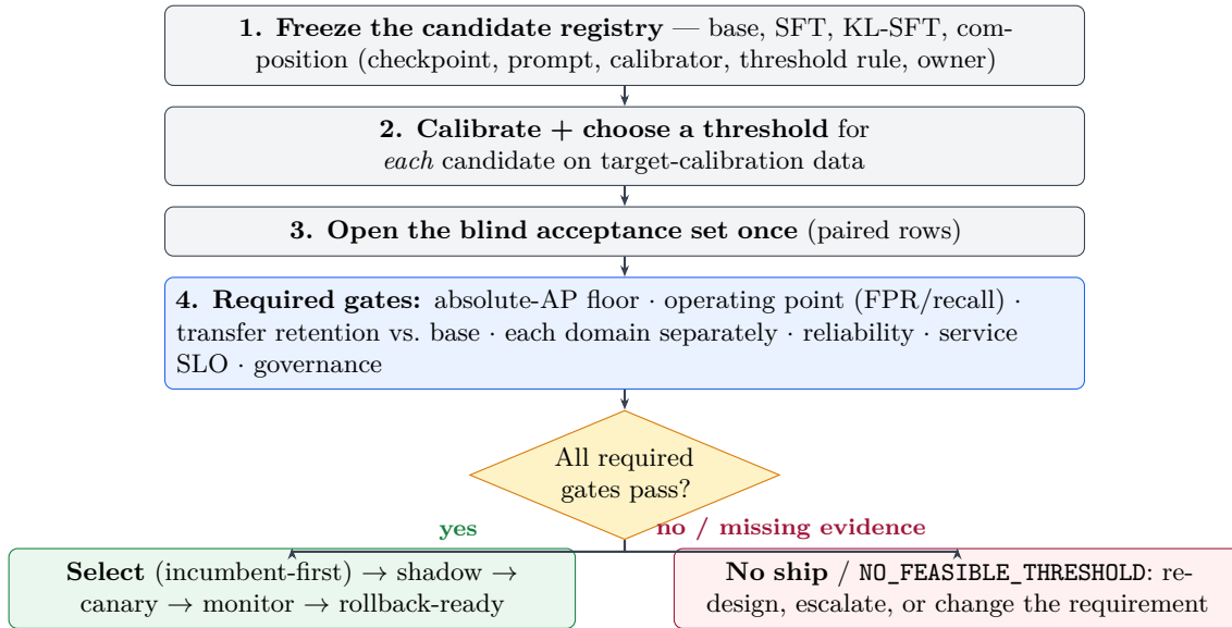
Figure 12: Gate candidates, not leaderboards (recommended workflow; not validated end to end by this study). Every candidate is calibrated and thresholded separately, evaluated once on a blind acceptance set, and must clear all required gates; a missing required gate is a failure, and an empty feasible set is a deliberate NO-SHIP, not a relaxed cutoff.
