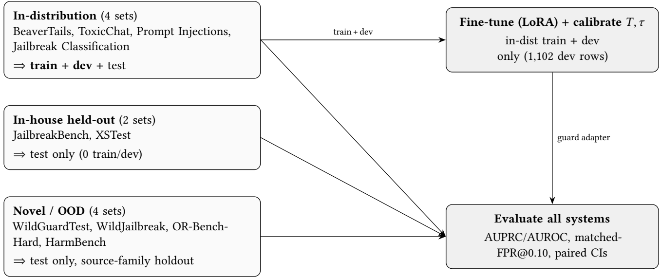
Figure 3: Benchmark pools and the train/dev/test separation. Only the four in-distribution sets feed fine-tuning and calibration (train + dev); the two in-house-held-out and four novel sets are test-only, so held-out and out-of-distribution evaluation measure transfer rather than memorization.
