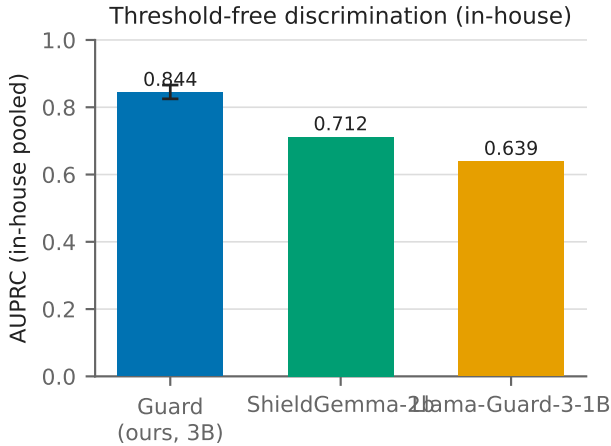
Figure 4: Pooled in-house AUPRC (2,018 test rows): the guard (0.844) leads ShieldGemma-2b (0.712) and Llama-Guard-3-1B (0.639) on point estimates.
