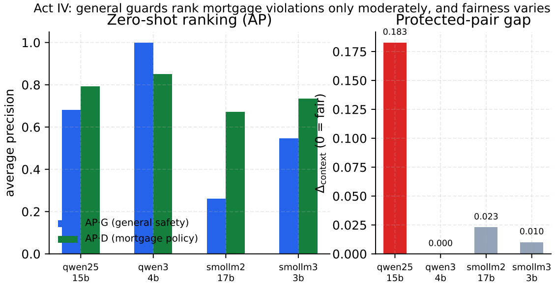
Figure 6: Zero-shot base guards on the mortgage benchmark: ranking (AP·G, AP·D; left) and the protected-pair fairness gap \Delta_{\text{context}} (right). AP·D is only moderate, and \Delta_{\text{context}} separates guards that AP alone rates similarly (Qwen2.5-1.5B’s 0.183 gap vs. Qwen3-4B’s 0).
