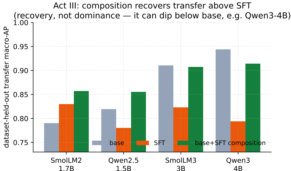
Figure 3: Per-checkpoint transfer macro-AP for base, SFT, and the base+SFT composition. Composition (green) exceeds SFT (orange) for every checkpoint, and lands at or above base except for the strongest base (Qwen3-4B) — transfer recovery , not Pareto dominance.
