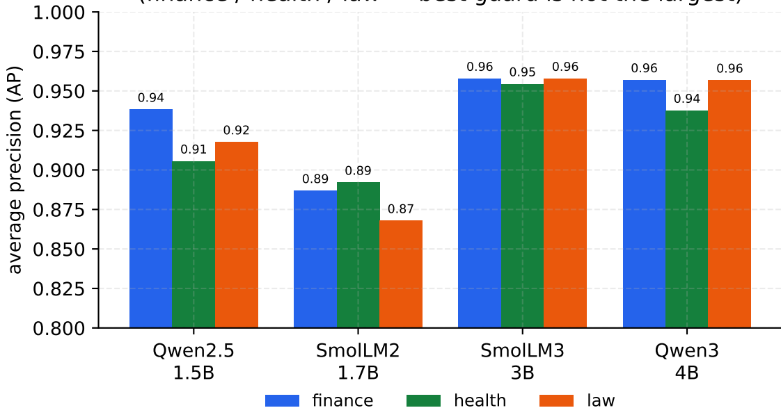
Act IV breadth: zero-shot base guards on ExpGuard (finance / health / law --- best guard is not the largest)
