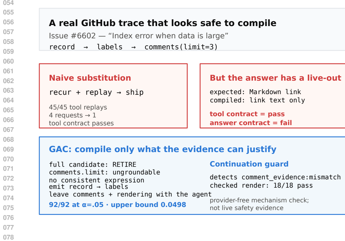
Figure 1: A real-record example of guarded compilation: recurring tool names identify a candidate, but an ungroundable argument and a downstream continuation contract can still require refusal or fallback.
