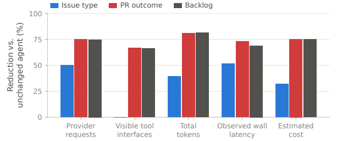
Figure 4: Per-family reduction against the unchanged agent. The issue-type family is the low end of every metric because its groundability proof admits only a two-read prefix and leaves the third read – and the interface – with the agent.
