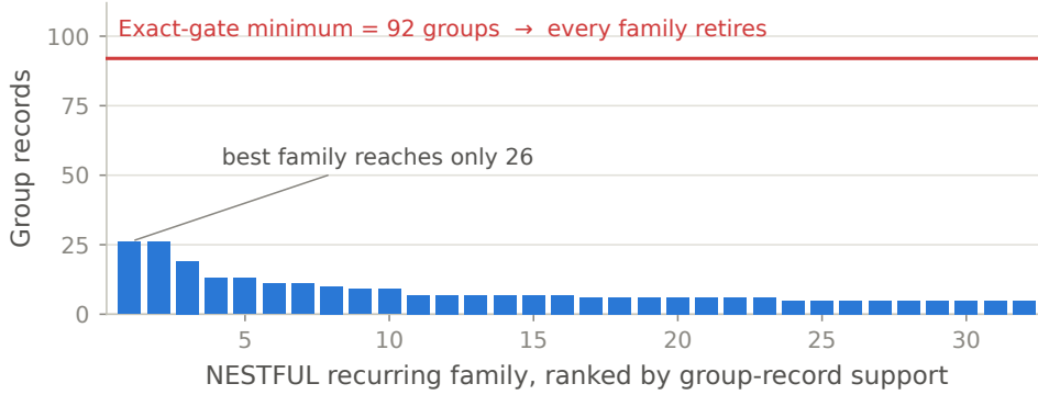
Figure 6: NESTFUL family supports against the 92-group requirement implied by eq. (7) at \alpha = 0.05 , \delta = 0.1 , |\Lambda| = 11 . The largest family reaches 26 groups, so every family retires at calibration even though provenance, synthesis, and replay all succeeded.
