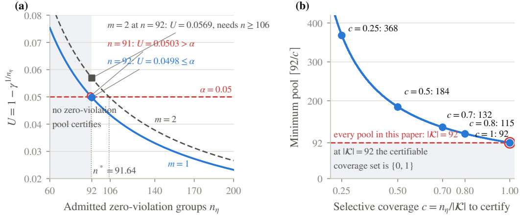
Figure 4: Why a 92-group pool certifies only full coverage. Left: the zero-violation bound U(n) = 1 - (\delta/|\Lambda|)^{1/n} at \delta = 0.1 , |\Lambda| = 11 crosses \alpha = 0.05 between n = 91 (0.0503) and n = 92 (0.0498). Right: the smallest pool \lceil 92/c \rceil that can certify selective coverage c ; every calibration pool in this paper is 92, so the certifiable coverages are 0 and 1 whatever q ranks.
