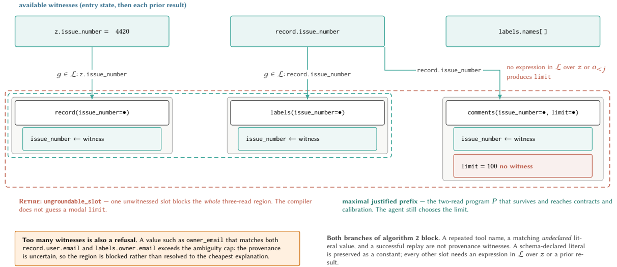
Figure 3: Equation (1) applied to the held-out issue-4420 record. Each nonliteral argument slot needs an expression in L over the entry state or a prior result; the green edges carry that expression, and the limit socket has no incoming edge at all. The diagram therefore asks a strictly harder question than recurrence: not “did this sequence repeat?” but “can every socket be wired from an allowed prior value?” One unwitnessed slot retires the whole three-read region, and a slot with too many witnesses does the same — both branches of algorithm 2 block rather than resolving to the cheapest available explanation. The ambiguity inset is illustrative; the wiring and the refusal are the executed compiler’s decision on that record.
