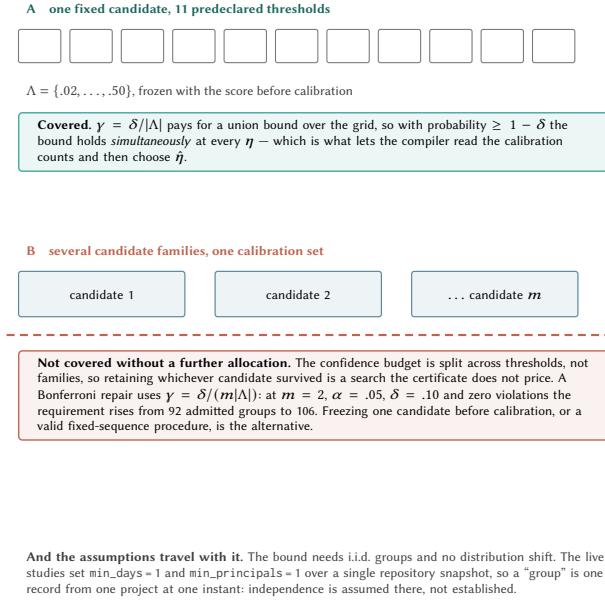
Figure 12: What the proposition licenses, and what it does not. (A) One fixed candidate against the predeclared grid is covered: \gamma = \delta/|\Lambda| buys a bound that holds simultaneously at every \eta , which is what permits reading the calibration counts before choosing \hat{\eta} . (B) Several candidates sharing one calibration set is a search the certificate does not price, and the assumptions travel with the fence: the live configuration makes group independence an assumption the snapshot can not verify.
