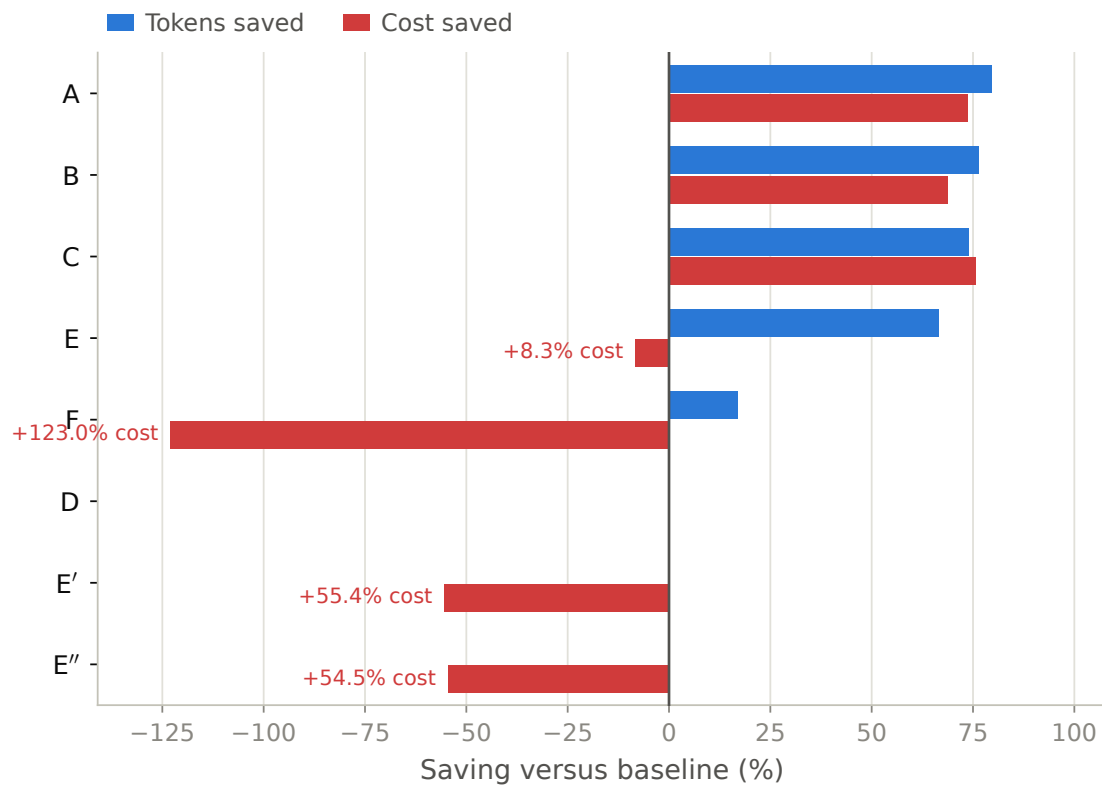
Figure 4. Controlled demonstration suite. Three of the eight conditions are negative controls whose only correct outcome is no compaction, and two of the compacting rows cost more than their baselines once prompt-cache reuse is fragmented.
