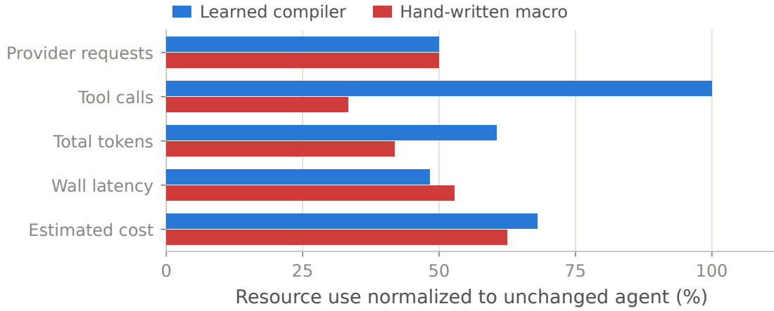
Figure 5. The live comparison that constrains the contribution, on the 30-pair expanded replication. The hand-written macro is at or below the compiled condition on every resource except observed wall latency, and uses one tool call where the compiler keeps three.
