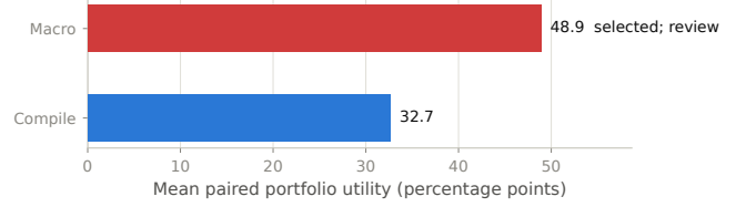
Figure 20: The frozen selection, taken over the 30 independent calibration issues. Both actions clear the risk limits, so the decision is made on mean paired utility alone and the measured macro wins it. Selection routes the action to human review; it does not deploy it.
