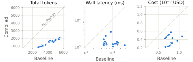
Figure 17: The same 18 pairs, unaggregated. Every issue is one point, baseline against compiled, so the reduction is visible as a distribution rather than a mean: no pair crosses the no-change diagonal on any of the three endpoints. Latency is plotted on log axes because the baseline spans an order of magnitude.
