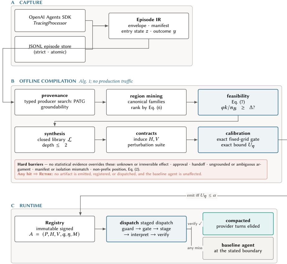
Figure 6: System architecture of GAC. (A) Capture normalizes framework traces into one typed Episode IR. (B) Offline compilation touches no production traffic and is a cascade of independent rejection points; the shaded barrier band lists conditions under which no statistical evidence can license an artifact. (C) Runtime resolves at the entry boundary. Of the terminal runtime edges, exactly one produces a compacted execution; every clean rejection returns the baseline and any failure whose reversibility cannot be attested raises an incident. “Baseline” is exact only where a staging owner holds the commit boundary: the outer runner can restore byte-identical model input, whereas the model-boundary adapter cannot un-emit a response the host has already committed to history (section 3.8.1).
