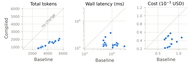
Figure 17: The same 18 pairs, unaggregated. Every issue is one point, baseline against compiled, so the reduction is visible as a distribution rather than a mean: no pair crosses the no-change diagonal on any of the three endpoints. Latency is plotted on log axes because the baseline spans an order of magnitude.
