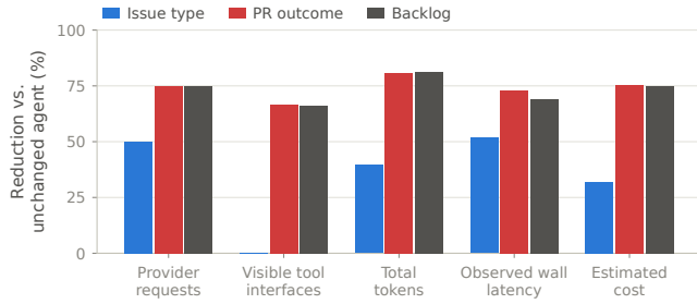
Figure 15: Per-family reduction against the unchanged agent. The issue-type family is the low end of every metric because its groundability proof admits only a two-read prefix and leaves the third read – and the interface – with the agent.
