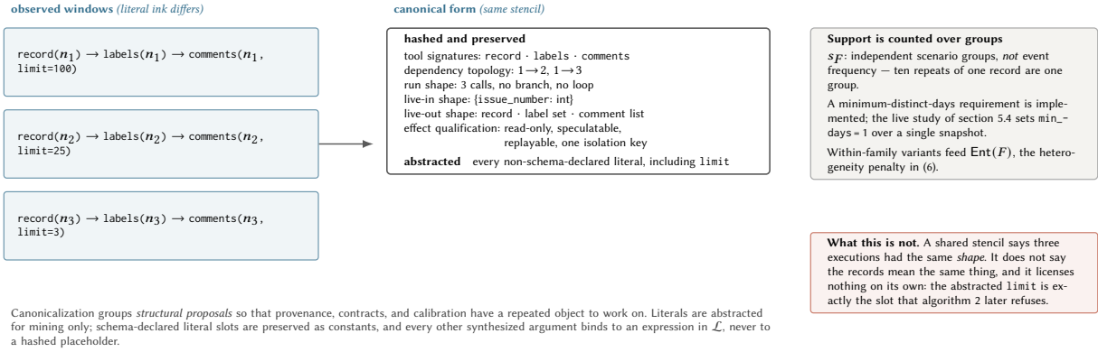
Figure 7: What a canonical family is, and what it is not. Hashing the tool signatures, dependency topology, run shape, and live-in/out shape while abstracting literals groups structural proposals so that provenance, contracts, and calibration have a repeated object to work on. Support is counted across independent scenario groups rather than by event frequency. A shared stencil is not evidence that the records mean the same thing, and it licenses nothing on its own: the abstracted limit is exactly the slot algorithm 2 goes on to refuse. The three observed windows are written with symbolic identifiers because only issue 4420 is a reported held-out record.
