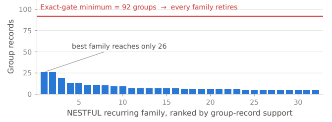
Figure 14: All NESTFUL families fall below the 92-group exact-gate requirement; the GitHub study was deliberately sized to reach it.
