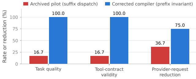
Figure 21: Why position is an invariant and not a tuning parameter. The archived pilot dispatched a compiled region from the wrong boundary and still reduced provider requests, which is exactly what makes it dangerous: efficiency survived while task quality and tool-contract validity collapsed to 16.7%. An optimizer scored on reduction alone would have accepted it.
