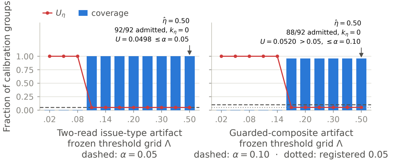
Figure 11: Fixed-grid selection on two sealed gates, from frozen grid to counts (n_\eta, k_\eta) to the bound U_\eta to the admitted threshold. Coverage and U_\eta are both fractions, so they share one axis. Left: the two-read issue-type artifact. It is degenerate — it admits every calibration group as soon as it admits any — and clears the registered budget. Right: the guarded-composite artifact, the only gate here that rejects groups at its selected threshold; the same selectivity puts n below the 92 a zero-violation 5% bound needs, so its bound is 0.0520 and it is admitted only at \alpha = .10 . Zero observed violations never produces a zero bound: \gamma = \delta/|\Lambda| pays for the union bound over the grid, and reading the counts before choosing \hat{\eta} is legitimate only because the candidate, the score, and the grid were frozen first.
