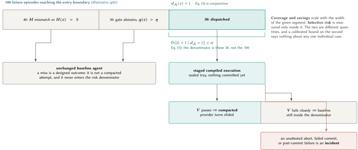
Figure 5: The population that (3) and (5) quantify over, and the slice the risk constraint conditions on. Savings are earned across the dispatched segment, while selective risk is measured inside it: an episode that misses on the manifest, the guard, or the gate returns the baseline and never enters the denominator, so it is not a compacted failure. A staged failure caught before the commit line also returns the baseline, but it does stay in the denominator, and only a post-commit dirty failure is an incident. The 40/30/30 split is illustrative and is drawn only to separate the two quantities; no coverage rate is claimed here.
