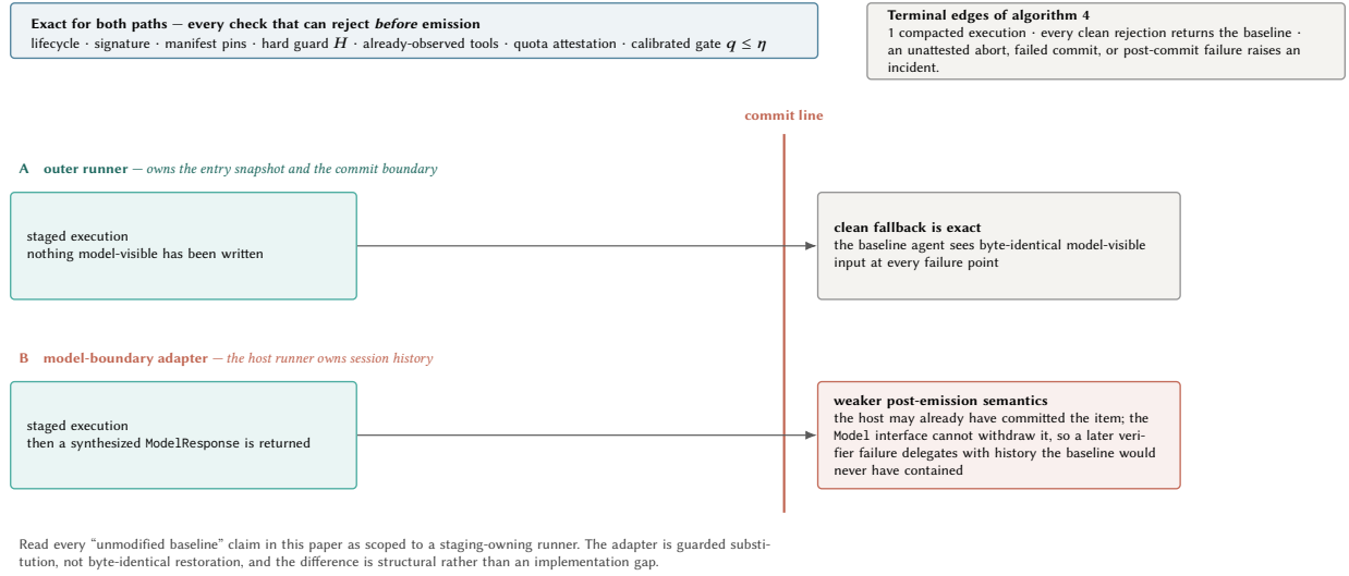
Figure 13: Where “the baseline runs unchanged” is exact. Both integration paths share every check that can reject before emission, so those rejections are exact for both. They differ only to the right of the commit line: the outer runner owns the entry snapshot and can restore byte-identical model-visible input, while the model-boundary adapter cannot withdraw a ModelResponse the host may already have committed to session history. The difference is structural rather than an implementation gap, and it is why one terminal edge of algorithm 4 raises an incident instead of reporting a fallback.
