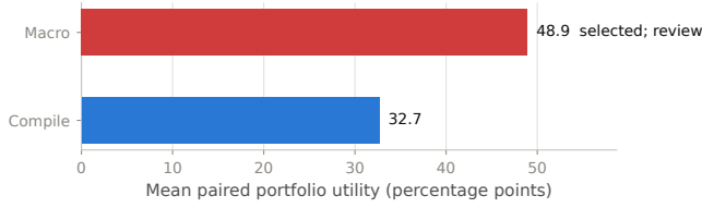
Figure 20: The frozen selection, taken over the 30 independent calibration issues. Both actions clear the risk limits, so the decision is made on mean paired utility alone and the measured macro wins it. Selection routes the action to human review; it does not deploy it.
