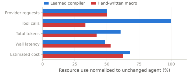
Figure 19: The live comparison that constrains the contribution, on the 30-pair expanded replication. The hand-written macro is at or below the compiled condition on every resource except observed wall latency, and uses one tool call where the compiler keeps three.
