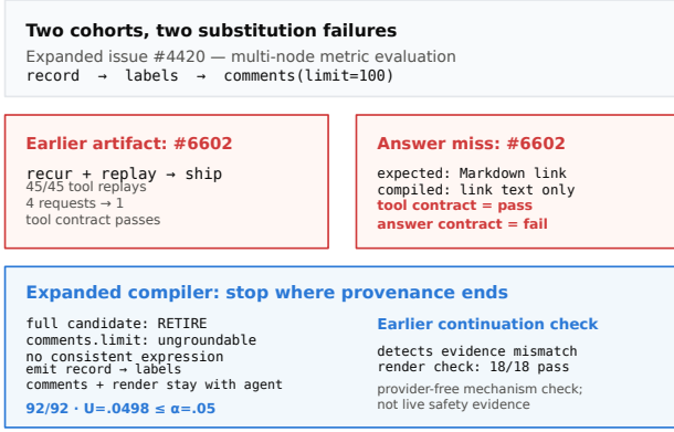
Figure 1: Why recurrence and tool replay do not license full substitution. In the expanded cohort, the comments limit varies and is not trace-groundable; the compiler therefore emits two reads and admits them under 92/92 calibration groups at \alpha = .05 . In a separate earlier cohort, a three-read artifact replayed tools cleanly but lost the URL on issue 6602; a provider-free continuation guard detected and checked-rendered the miss.
