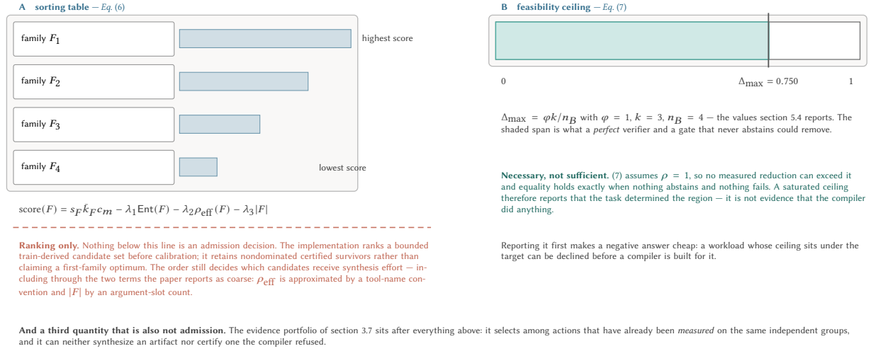
Figure 8: Two pre-synthesis questions, neither of which is admission. (A) Equation (6) orders candidates so that synthesis effort goes somewhere useful. It affects which fixed candidates are tried, but no admission decision reads it and the compiler retains nondominated calibrated survivors rather than claiming a first-family optimum. (B) Equation (7) bounds what a perfect verifier and a never-abstaining gate could remove. It is necessary, not sufficient: a saturated ceiling reports that the task determined the region rather than that the compiler succeeded. The gauge is drawn at the values section 5.4 reports.
