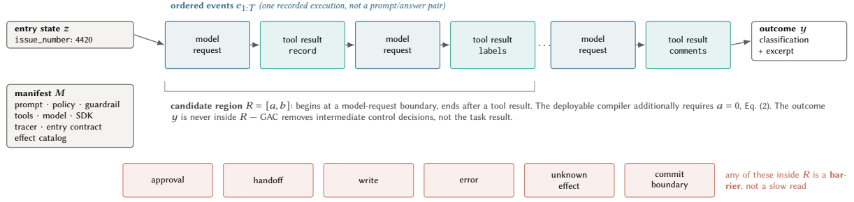
Figure 2: Anatomy of one episode, and of a candidate region inside it. An episode is a typed, version-pinned execution record rather than a prompt/answer pair: the manifest M pins the identities a learned artifact may later be reused under, and the events e_{1:T} retain the tool receipts a compiler would have to reconstruct arguments from. A candidate region is a bounded segment of that record, and it never contains the outcome y . The icons in the lower strip are examples of event kinds that act as barriers; they are not an exhaustive state machine.
