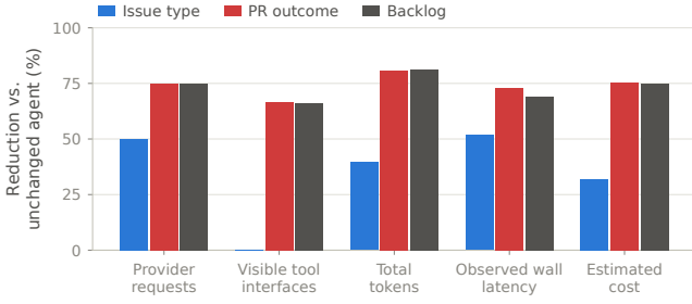
Figure 15: Per-family reduction against the unchanged agent. The issue-type family is the low end of every metric because its groundability proof admits only a two-read prefix and leaves the third read – and the interface – with the agent.
