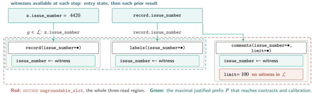
Figure 2: Equation (1) on the held-out issue-4420 record: both issue_number slots have an expression in \mathcal{L} over the entry state or a prior result; the limit literal varies across the supporting traces (100 in 130 of 132, 1 in two) and has none, so the three-read region retires and only the two-read prefix is emitted.
