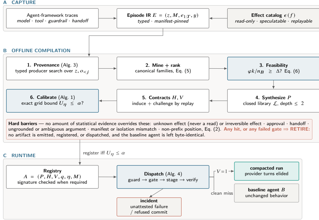
Figure 1: Architecture of GAC. (A) Capture normalizes traces into one typed Episode IR against a declared effect catalog. (B) Compilation is a cascade of independent rejection points; the shaded band lists barriers no statistical evidence can override. (C) At runtime one terminal edge compacts; clean rejections return the unchanged agent, and unattested failures raise an incident.
