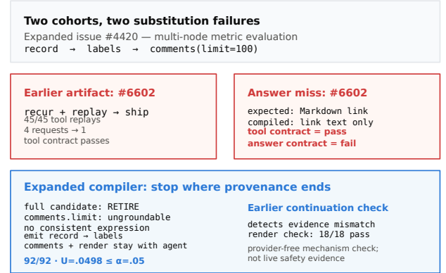
Figure 1: Why recurrence and tool replay do not license full substitution. In the expanded cohort, the comments limit varies and is not trace-groundable; the compiler therefore emits two reads and admits them under 92/92 calibration groups at \alpha = .05 . In a separate earlier cohort, a three-read artifact replayed tools cleanly but lost the URL on issue 6602; a provider-free continuation guard detected and checked-rendered the miss.
