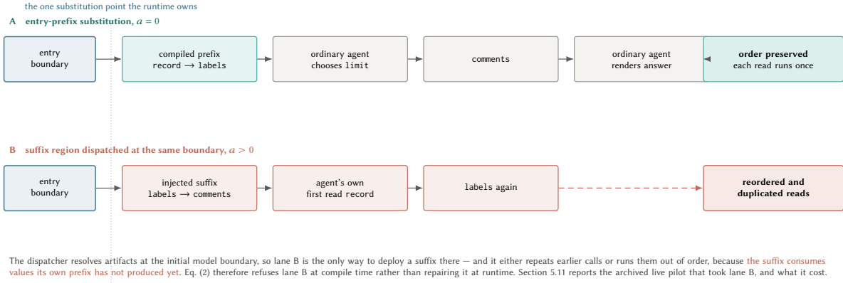
Figure 4: Why prefix-only, drawn as the two orders the runtime can actually produce. Because resolution happens at the initial model boundary, a region with \alpha > 0 can only be deployed by injecting it there, which either repeats reads the agent will make anyway or runs them before the values they depend on exist. This panel depicts the current runtime placement and carries no measurement: the archived live pilot that took the lower lane, and what it cost, is reported in section 5.11.
