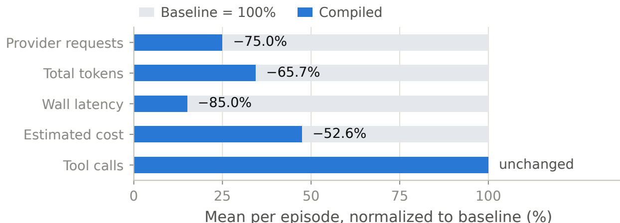
Figure 16: Prescribed-prefix ablation, 18 held-out pairs, each mean normalized to its own unchanged baseline. Tool calls are the control: the compiled program performs the same three reads, so what falls is the model-mediated control flow around them, not the work. Per-metric absolute means and Wilcoxon p -values are in table 19.
