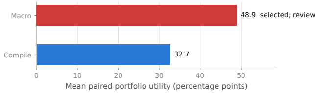
Figure 9: The frozen selection, taken over the 30 independent calibration issues. Both actions clear the risk limits, so the decision is made on mean paired utility alone and the measured macro wins it. Selection routes the action to human review; it does not deploy it.
