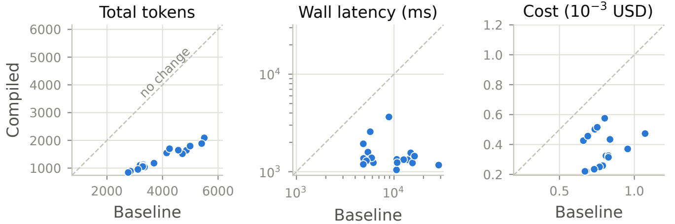
Figure 5: Per-issue paired measurements. All points fall below the no-change diagonal for total tokens, wall latency, and estimated cost.
