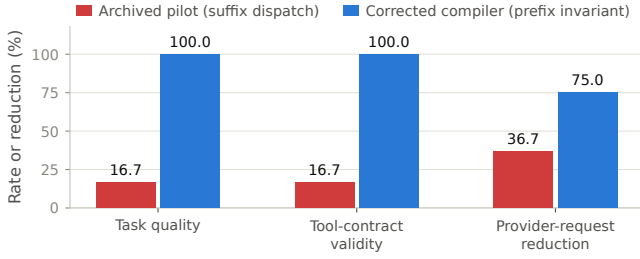
Figure 8: Safety ablation from the archived pilot. Request savings without correct execution position are not an acceptable optimization.
