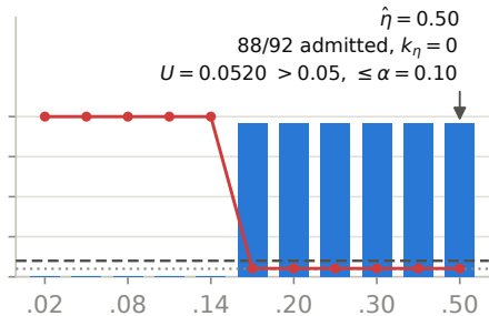
Guarded-composite artifact frozen threshold grid \Lambda dashed: \alpha = 0.10 · dotted: registered 0.05
